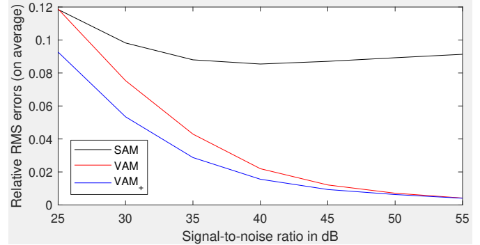
Fig. 5. The average of the relative RMS errors of phase retrieval over 75 experiments is presented for 7 different levels of Gaussian noise. VAM + (the blue curve) is clearly superior to VAM (the red curve) and SAM (the black curve). The quality of phase retrieval by VAM and SAM for SNR 25 dB is at the same level but the difference becomes more substantial for higher SNR. The relative RMS error of VAM + and VAM shapely decreases for higher SNR while that of SAM remains high (above 8.5%) for all SNR due to model deviations.
