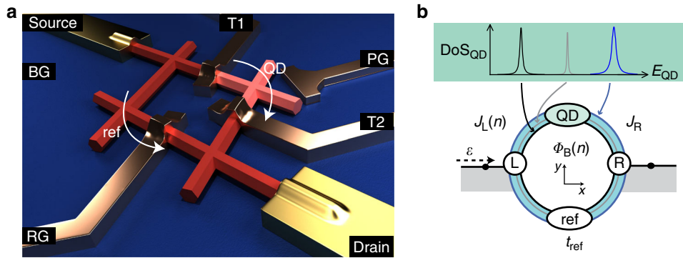
Fig. 6 The multi-path interferometer. a Illustration of the device: in red the nanowire, in gold the leads, in copper the gates and in pink the quantum dot. b Schematic of the device: the quantum dot exhibits a density of states ( \text{DoS}_{\text{QD}} ) comprised of discrete levels with distinct energy broadening. In the model, we assume that the dot states might couple to different interferometer trajectories that are sketched as rings of different colour.
