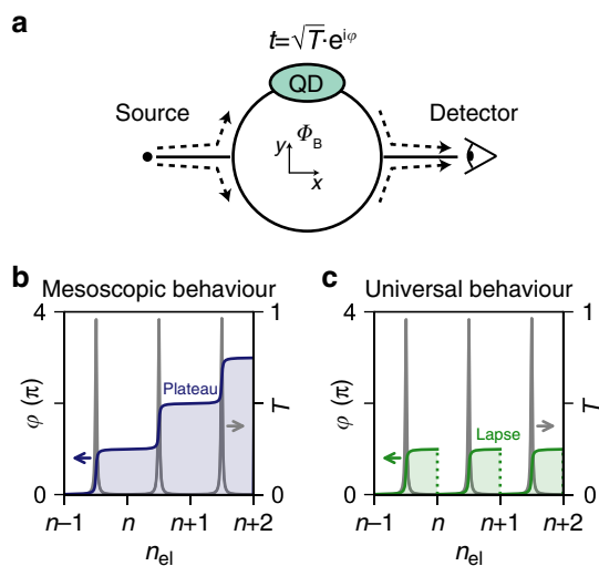
Fig. 1 Mesoscopic and universal phase behaviours. a The minimum setup to study the transmission phase via a quantum dot (in light green) is a two-path interferometer. b, c Transmission phase \varphi and probability T as a function of the electron number n_{el} in a quantum dot. A Breit–Wigner function describes each of the resonances (in grey). b The mesoscopic regime: phase plateaus in the Coulomb valleys appear at 0 and \pi . c The universal regime: phase lapses occur between transmission resonances.
