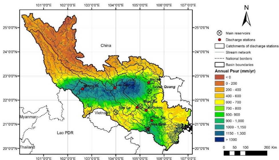
Figure 3.8. Annual average rainfall surplus in the Red River Basin for the period 2003 – 2012. Also indicated are the largest dams that provide opportunities for water storage. Hòa Bình and Thác Bả dam were operational during this entire period, Tuyen Quang and Son La dam were commissioned in 2008 and 2011, respectively.
