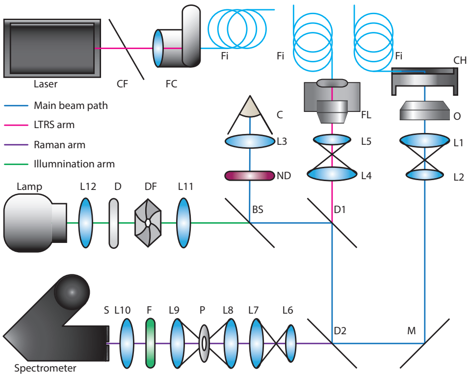
Figure 5.2: Experimental setup used in this chapter. (blue) The main beam path. (red) The LTRS arm. (purple) The Raman arm. (green) The illumination arm. Components: L1-12 - lenses, CF - clean-up filter, FC - Newport 9131-M fibre coupler, Fi - Thorlabs PM-630-HP polarisation maintaining fibre, FL - fibre launcher, C - camera, ND - neutral density filters, Lamp - halogen lamp, D - diffuser plate, DF - diaphragm, BS - 50:50 beam splitter, D1, D2: dichroic mirror, M - silver mirror, O - Olympus UPLSAPO 60XW or LUMPLFLN 40XW objective, CH - chip holder, F - filter, P - pinhole \phi=100\ \mu\text{m} , S - spectrometer entrance slit, spectrometer Acton LS 785. Lens sets L1/L2, L4/L5 and L6/L7 form beam expanders. L9, P and L8 form a confocal filter.
