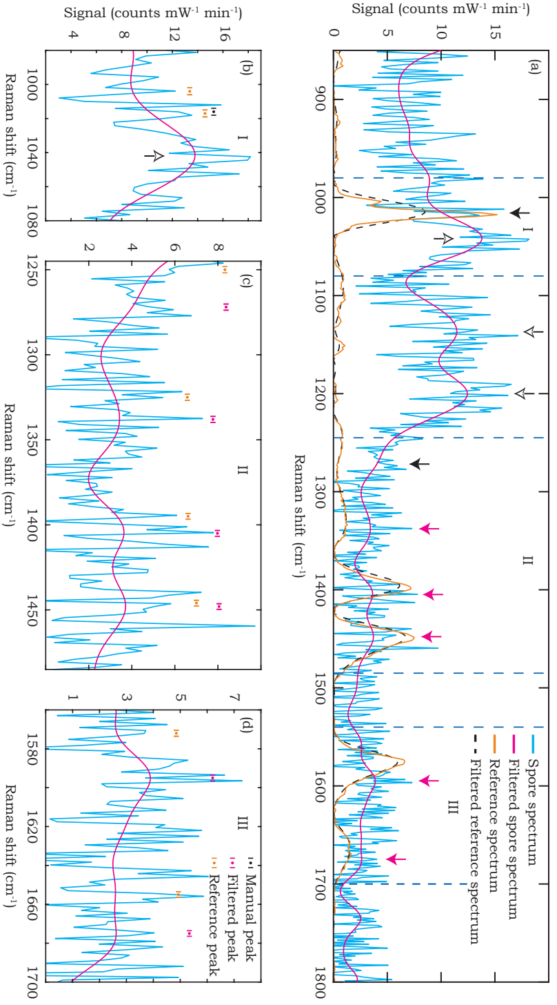
Figure 5.5: Figure 14 Few spores Raman spectrum from the 10 \mu\text{m} trap. (a) Full spectrum with five assigned peaks (magenta arrows), two manually assigned peaks (black arrows) and three background peaks (open arrows). (b) Close up, showing the peaks at 1016 and 1042 \text{cm}^{-1} . (c) Close up, showing the spore peaks at 1338, 1405 and 1448 \text{cm}^{-1} . (d) Close up, showing the assigned peaks at 1572 and 1655 \text{cm}^{-1} . The bars in plots (b-d) give the local spectrometer resolution at the position of the manually assigned peaks, the assigned peaks and the reference peaks.
