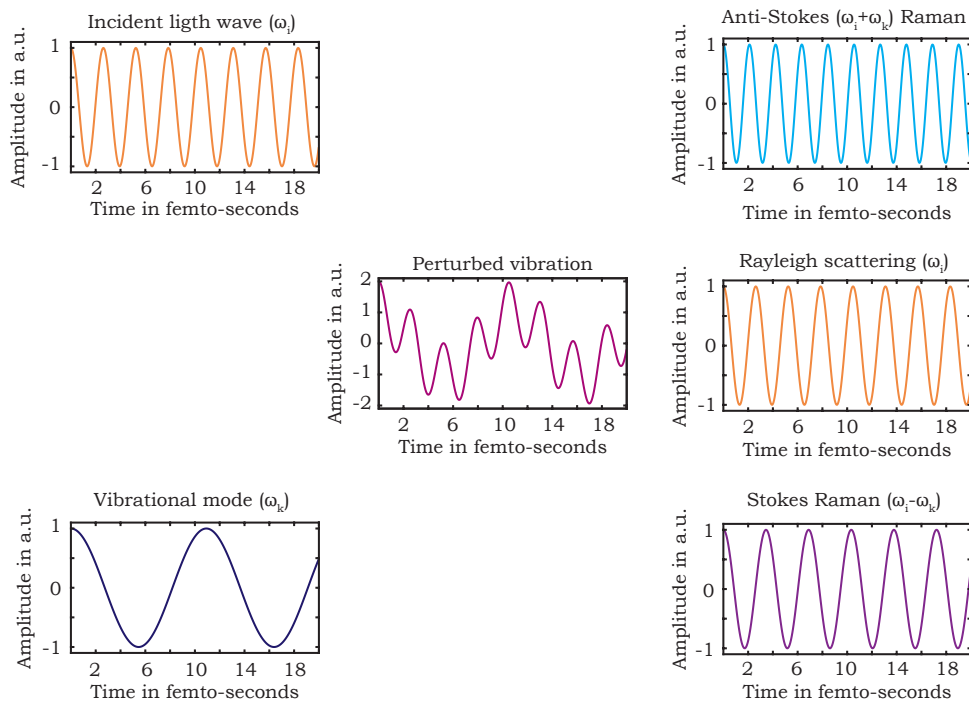
Figure 1.1: Graphical representation of the frequencies involved in Raman scattering. An incident light wave, in this case with a wavelength of 785 nm (top left graph) interacts with a vibrational mode of a molecule, in this case the CH stretch mode (Wilson Number 2) of polystyrene (bottom left graph). This interaction induces a dipole oscillation in the molecule, which resembles the vibrational mode perturbed by the incident light wave (central graph). The oscillating dipole can radiate at two of three different frequencies. In the case that the vibrational mode was already populated the emitted light will have the sum frequency (top right graph) if the vibrational mode is relaxed which is called Anti-Stokes Raman scattering or the same frequency as the incident light (middle right graph) if the vibrational mode remains populated which is called Rayleigh scattering. In the case that the vibrational is mode is not populated at the moment of the interaction, the incident light will be either Rayleigh scattered or will have the difference frequency (bottom right graph) if the vibrational mode is excited which is called Stokes Raman scattering.
