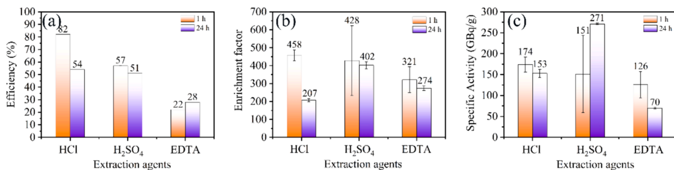
Fig. 5. (a) Efficiency, (b) enrichment factor and (c) specific activity of ^{51}\text{Cr} extracted with different extracting solutions (30% HCl, 15% \text{H}_2\text{SO}_4 and EDTA (1 mM, pH = 5)) at different extraction times from irradiated MIL-100 (Cr).
