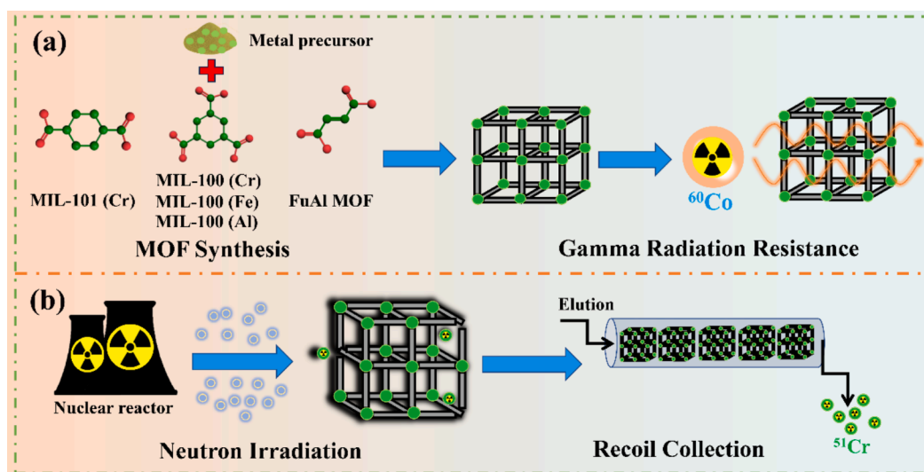
Fig. 1. Schematic diagram of (a) gamma radiation stability of five MOFs and (b) high specific activity ^{51}\text{Cr} production.
