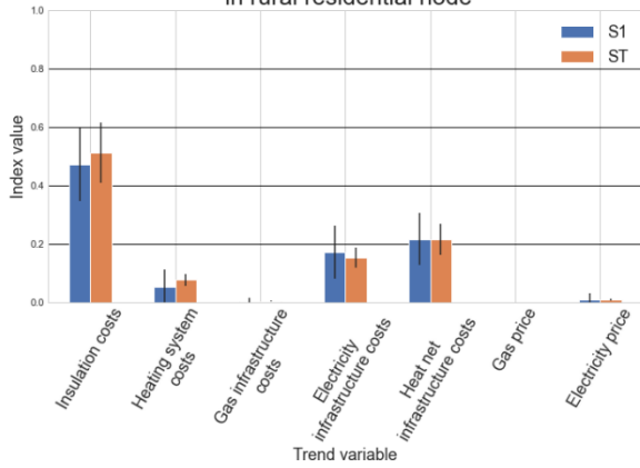
Sobol indices for LT heat net in rural residential node
