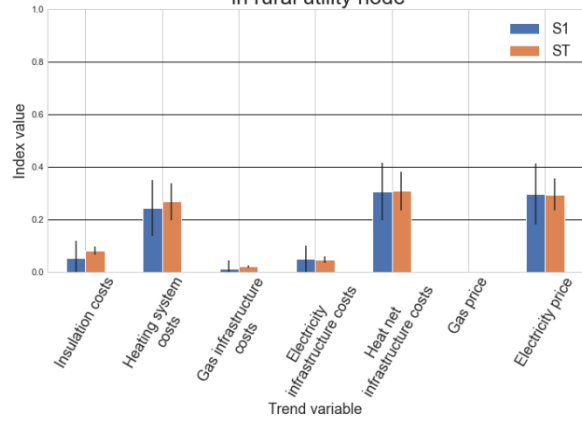
Sobol indices for LT heat net in rural utility node
