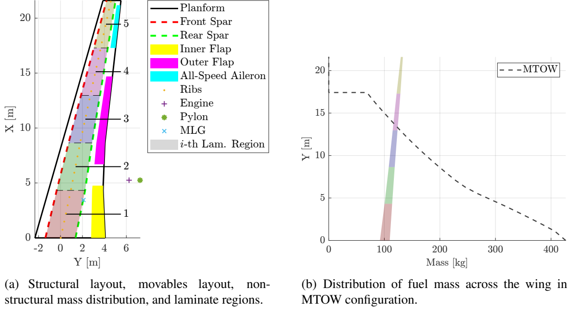
Figure 2: Visual representation of the SE 2 A MR wing.
