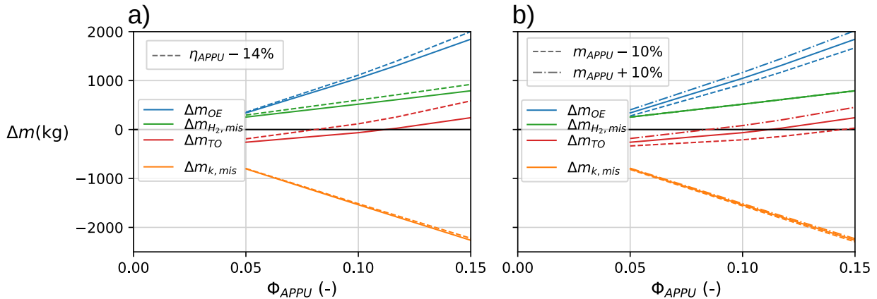
Figure 5 – Sensitivity of the overall aircraft masses and mission fuel burn to APPU efficiency (left), assuming that the engine delivers equal thrust but has increased fuel consumption), and APPU engine mass (right).
