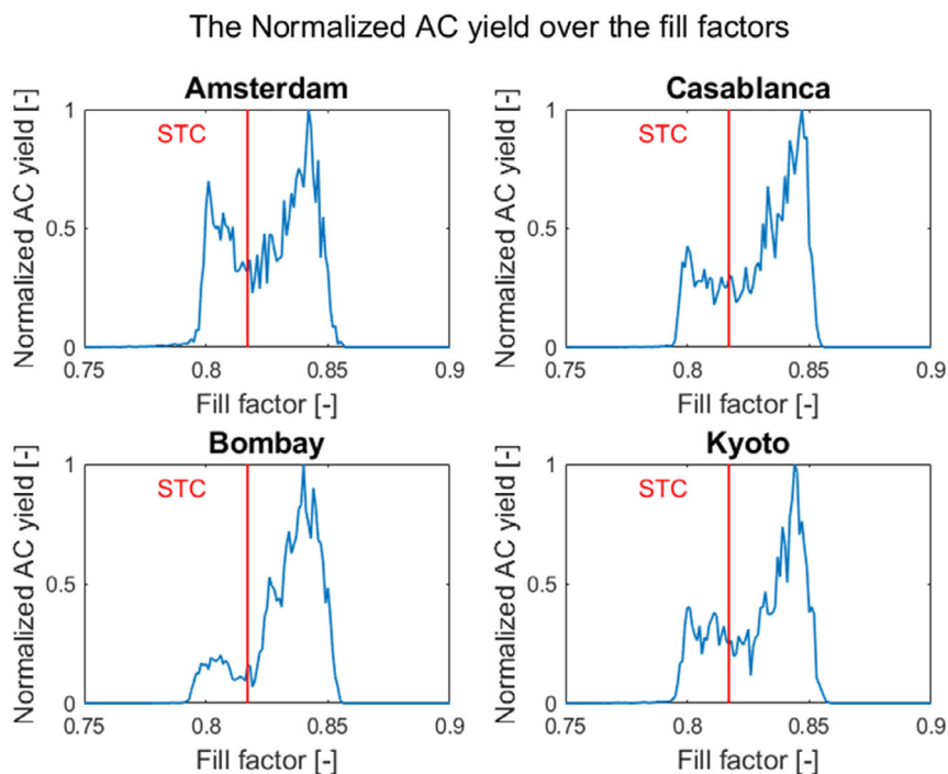
Figure 6. The relative AC energy yield for each fill factor. The red line indicates the fill factor at STC. It shows that at each location, most of the AC electricity is generated at a higher fill factor than the fill factor at STC.
