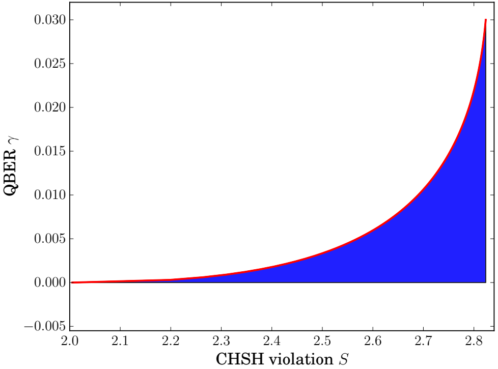
Figure 3.3: QBER \gamma allowed in function of the CHSH violation S obtained in the testing procedure when n \rightarrow \infty and d finite. The blue region is the secure region i.e. the region where the bound B'(n, d, \zeta, \gamma) decays exponentially in n for a fixed d .
