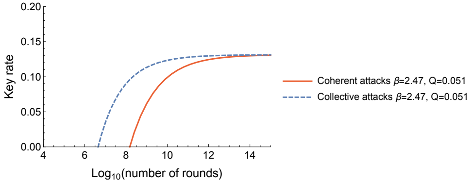
Figure 5.4: Key rates vs logarithm of the number of rounds n for parameters that are readily-implementable in NV centres setups (CHSH violation S = 2.47 and QBER Q = 0.051 ). The red line shows the key rates obtained against general coherent attacks, and the blue dashed line shows the key rates under the assumption of collective attacks. The security parameters are chosen to be \epsilon_{DIQKD}^c = 10^{-2} and \epsilon_{DIQKD}^s = 10^{-5} .
