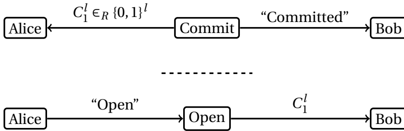
Figure 2.3: Ideal Randomized String Commitment. In the first part Alice gets a random l -bit string C_1^l \in \{0, 1\}^l , and Bob is notified that the string is committed. In the second phase, Alice asks ‘‘the box’’ to reveal the string to Bob.
