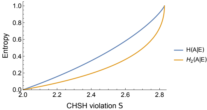
Figure 5.7: Graph illustrating the difference of the conditional von Neumann entropy H(A|E) and the conditional collision entropy H_2(A|E) as a function of the CHSH violation S .
