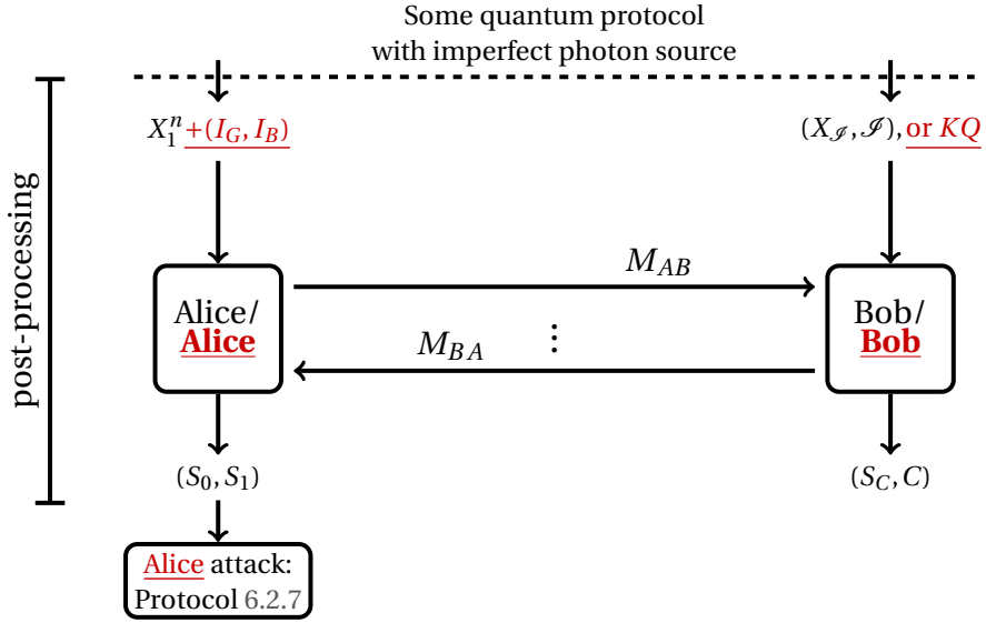
Figure 6.3: Schematic view of the classical post-processing between (dishonest) Alice and (dishonest) Bob. Before the post-processing Alice and Bob have run an unspecified quantum protocol which gave them their inputs: X_1^n + (I_G, I_B) for (dishonest) Alice, and (X_{\mathcal{S}}, \mathcal{S}) , or KQ for (dishonest) Bob. When Alice is dishonest, we will consider that she is “honest but curious” at the post-processing level, meaning that Alice will run the post-processing honestly with Bob, but she will record all communication M_{AB}, M_{BA} and use them at the end together with her extra-input (I_G, I_B) , to extract more information than what she should get out of the protocol. To do so she will use the strategy described in Protocol 6.2.7
