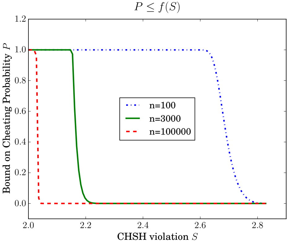
Figure 3.1: Security is possible for any violation of the CHSH inequality, but depending on the violation we need to send a larger number of qubits n .
