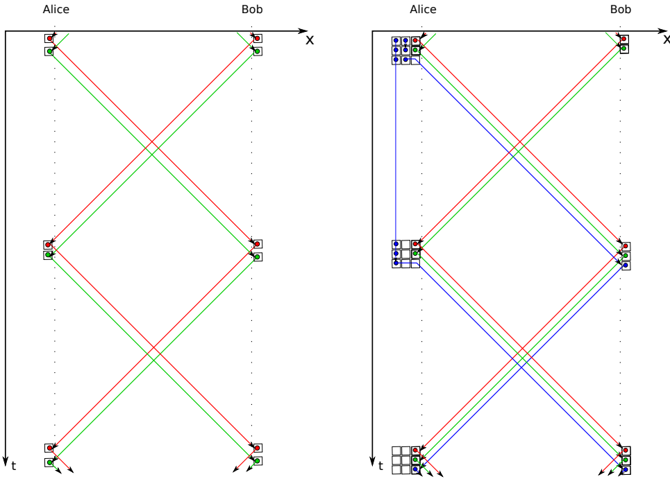
Figure 3.4: On the left hand side an illustration on how to store a certain number of qubits (here two EPR pairs, the red and the green pairs) in an arbitrary large quantum channel thanks to one qubit memory on each side. Alice and Bob keep forwarding each other their half of an entangled state in such a way that the state is preserved in the quantum channel. The right hand side figure illustrates how to create another EPR pair (here the blue EPR pair) using three qubits memory on Alice's side and one on Bob's side. These constructions works for an arbitrarily high amount of EPR pairs by iterating the procedure.
