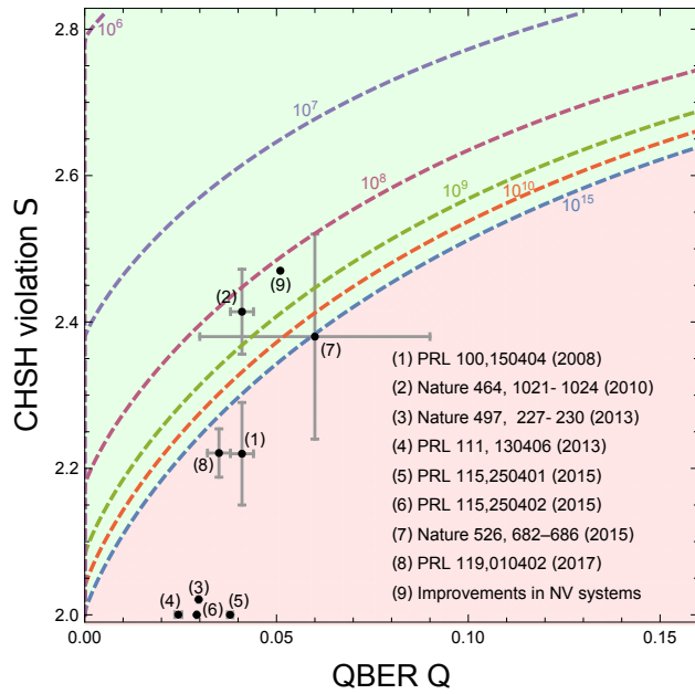
Figure 5.5: Region of positive key rates for coherent attacks : The red area is the region of values of QBER ( Q ) and CHSH violation ( S ) for which a positive key rate cannot be reached with any number of rounds. In the green area, the dashed curves represents the minimum number of rounds required to get positive key rate. For parameters above each curve, a key rate can be extracted if the number of rounds is higher than specified in the curve. The points show the Bell violation and estimated QBER achieved by previous experiments (see Table 5.4). They, however, do not reflect the corresponding entanglement generation rates. Similarly to [1], we take \epsilon_{DIQKD}^c = 10^{-2} and \epsilon_{DIQKD}^s = 10^{-5} .
