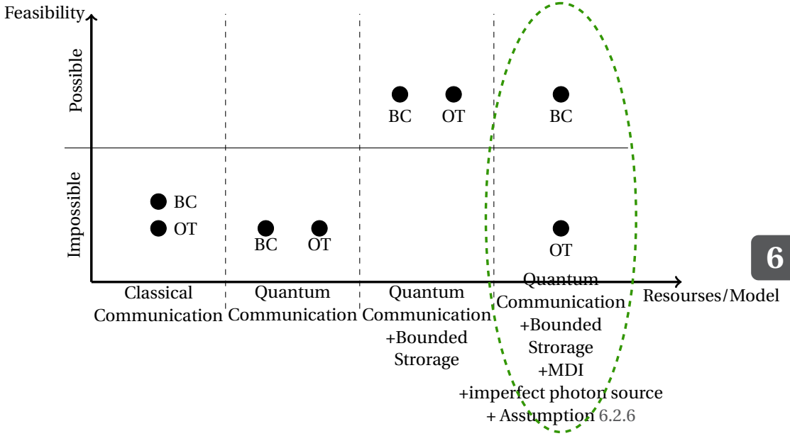
Figure 6.4: Schematic representation of the “Feasibility” of OT and BC depending on the resources/model used in the protocol. In the first column neither BC nor OT are possible, but since OT can be used in order to get BC but not the contrary, OT is somewhat a harder problem, which is why it is below BC. When quantum communication are possible then OT and BC are equivalent (represented at the same level) but still impossible. In the third column we add the Bounded Storage assumption, which makes both protocol possible. They are still equivalent. In the last column we add that quantum communication between the parties are made in the MDI settings, and we assume that the parties do not have perfect single photon source. In this case BC is possible (see Theorem 6.4.12) but OT is not (see Theorem 6.4.20).
