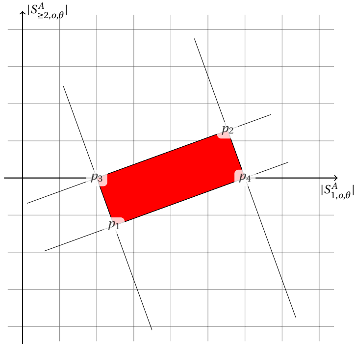
Figure 6.6: Each of the line is defined by one of the four inequalities in (6.56). The red region is the set of points that satisfies the four linear constraints from (6.56). Since we are optimizing a linear function with linear constraints, by linear programming we know that the optimum is reached for one of the four extreme points p_1, p_2, p_3, p_4 , which are at the intersection of the lines. In the particular case of this figure \min |S_{1, o, \theta}^A| is reached in p_3 .
