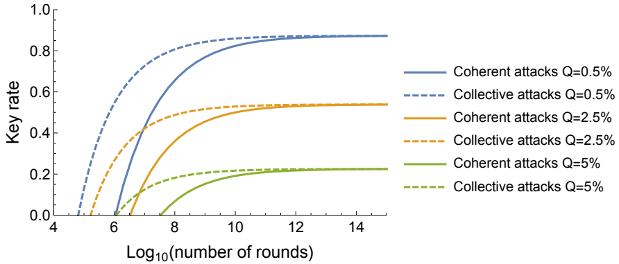
Figure 5.3: Key rates vs logarithm of the number of rounds for collective attacks (dashed lines) and coherent attacks (solid lines). The different curves represent different values of QBER Q = (0.5\%, 2.5\%, 5\%) considering an implementation where the maximally entangled state is subjected to depolarizing noise (see relation (5.12)). The security parameters are taken as \epsilon_{DIQKD}^c = 10^{-2} and \epsilon_{DIQKD}^s = 10^{-5} .
