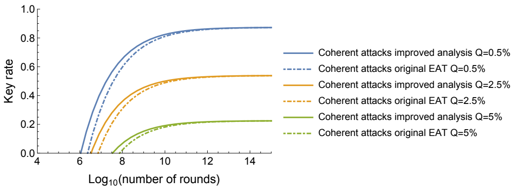
Figure 5.1: Key rate r vs logarithm of the number of rounds n . Comparison of the improvements in the key rate, for an implementation where the maximally entangled state is subjected to depolarizing noise and therefore S = 2\sqrt{2}(1 - 2Q) , for QBER Q = \{0.5\%, 2.5\%, 5\%\} . The dashed curves correspond to the key rates derived in the original analysis [1, 41], the solid lines represent the key rates derived in Theorem 5.2.2. Similarly to [1], we take \epsilon_{DIQD}^c = 10^{-2} and \epsilon_{DIQD}^s = 10^{-5} .
