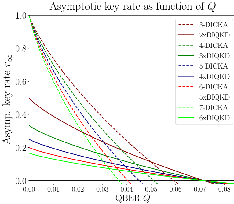
Figure 4.3: Asymptotic key rate for N -device-independent CKA (DICKA, dashed lines), and for the distribution of a secret key between N parties through N - 1 device-independent quantum key distribution ( (N - 1) \times DIQKD) protocols (solid lines), when each qubit experiences independent bit errors measured at a bit error rate (QBER) Q . From top to bottom, the lines correspond to N = \{3, 4, 5, 6, 7\} . We observe that for low noise it is advantageous to use our device-independent N -CKA protocol instead of using N - 1 DIQKD protocols [7]. In general, the comparison between the two methods depends on the cost and noisiness of producing GHZ states over pairwise EPR pairs.
