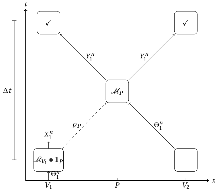
Figure 2.4: V_1 uses \Theta_1^n as an input to his device, which creates a bipartite state \rho_{AP} and sends the part \rho_P to the prover P , and measures the other part \rho_A to produce X_1^n \in \{0, 1\}^n as output. At the same time V_2 sends \Theta_1^n to P . When P receives the state and \Theta_1^n , he makes a measurement on the state and obtains Y_1^n \in \{0, 1\}^n . He sends Y to both verifiers. The verifiers check if Y_1^n = X_1^n (or if Y_1^n is "close enough" to X_1^n ), and measure the time it took to get back an answer from P .
