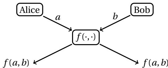
Figure 2.1: Schematic of a two-party computation. Each of the parties has an input, and they must compute the function f on these inputs, in a way that Alice never learns Bob's input and vice versa .
