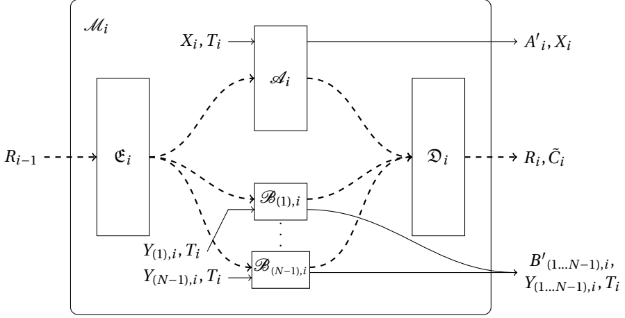
Figure 4.2: Description of the map \mathcal{M}_i . This map describes the round i of the first step of the Protocol 4.2.3. T_i is chosen at random such that P(T_i = 1) = \mu . X_i \in \{0, 1\} represents the “basis” in which Alice’s device, represented by the CPTP map \mathcal{A}_i , measures its input to get the output A'_i \in \{0, 1\} . X_i = 0 when T_i = 0 and X_i \in_R \{0, 1\} otherwise. Y_{(k),i} \in \{0, 1, 2\} represents the “basis” in which Bob _k ’s device, represented by the CPTP map \mathcal{B}_{(k),i} , measures its input to get the output B'_{(k),i} \in \{0, 1\} . If T_i = 0 we have Y_{(k),i} = 2 , else we have Y_{(k),i} \in_R \{0, 1\} . If T_i = 0 then \tilde{C}_i = \perp , else \tilde{C}_i = w_{\text{Parity-CHSH}}(A'_i, B'_{(1\dots N-1),i}, X_i, Y_{(1\dots N-1),i}) .
