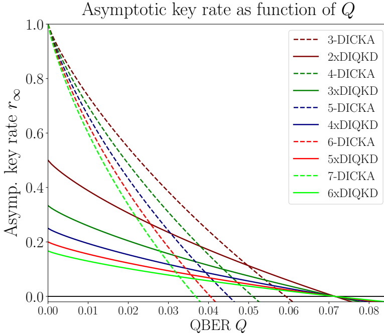
Figure 4.1: Asymptotic key rate for N -DICKA (dashed lines), and for the distribution of a secret key between N parties through N - 1 DIQKD protocols (solid lines), when each qubit experiences independent bit errors measured at a bit error rate (QBER) Q . From top to bottom, the lines correspond to N = \{3, 4, 5, 6, 7\} . We observe that for low noise regime it is advantageous to use DICKA instead of (N - 1) \times DIQKD [7]. In general, the comparison between the two methods depends on the cost and noisiness of producing GHZ states over pairwise EPR pairs.
