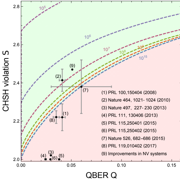
Figure 5.6: Region of positive key rates for collective attacks: The red area is the region of values of QBER ( Q ) and CHSH violation ( S ) for which a positive key rate cannot be reached with any number of rounds. In the green area, the dashed curves represents the minimum number of rounds required to get positive key rate. For parameters above each curve, a key rate can be extracted if the number of rounds is higher than specified in the curve. The points show the Bell violation and estimated QBER achieved by previous experiments (see Table 5.4). They, however, do not reflect the corresponding entanglement generation rates. Similarly to [1], we take \epsilon_{DIQKD}^c = 10^{-2} and \epsilon_{DIQKD}^s = 10^{-5} .
