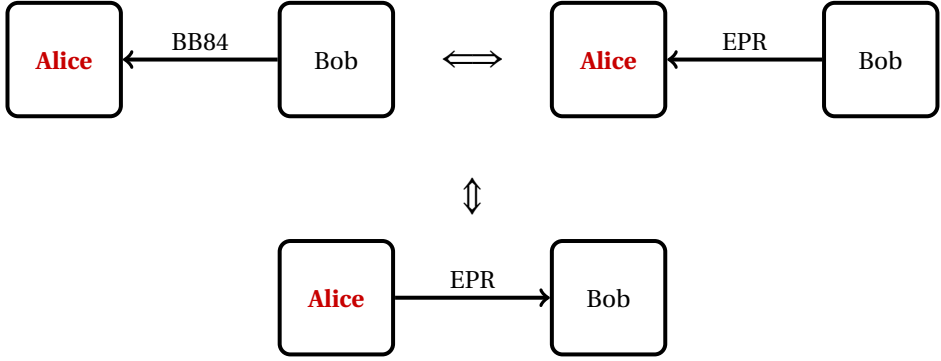
Figure 6.5: When honest Bob has access to a single photon source and Alice is dishonest, the three situations depicted are equivalent: In the first Bob chooses the bases \hat{\Theta}_1^n and \hat{X}_1^n uniformly at random, and sends a BB84 type state, as described in Protocol 6.2.2. The second picture depicts the equivalent scenario where he sends half of an EPR pair to Alice, and gets \hat{X} and \hat{\Theta} by measuring the other half. This scenario itself is equivalent to the last where it is (dishonest) Alice that sends half of the EPR pair. If some noise acts on the qubit sent by Bob to Alice in the first scenario, this can be seen as Alice applying a “noise map” on the half of the EPR pair she keeps before applying a measurement in the third scenario. In this virtual scenario, the other half of the EPR pair is assumed to be sent (measured) to (by) Bob without any noise.
