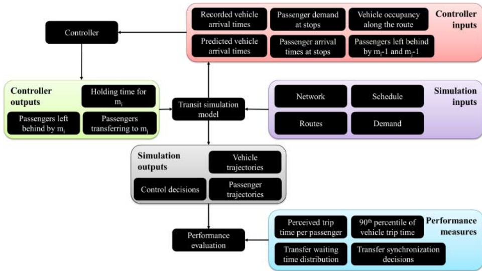
Figure 2. Schematic relations between the controller and the simulation model and the resulting key performance indicators.
