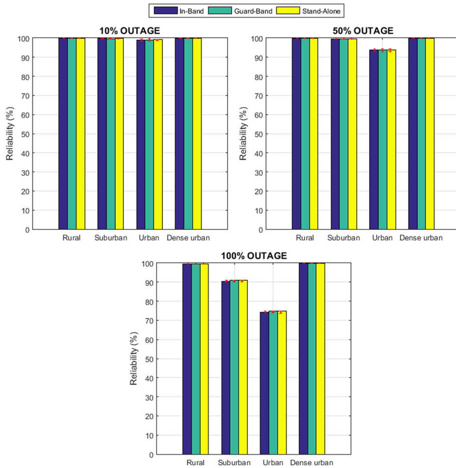
Fig. 7 Comparison of the reliability performance under the baseline configuration for different environments, outage percentages (10%, 50% and 100%) and for the three distinct NB-IoT deployment modes
