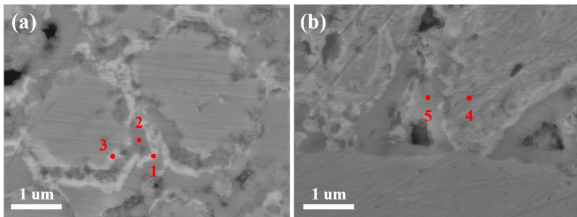
Fig. 12 SEM image of Cu@Ag sintered particle after 400 h aging: a SCu@Ag, b FCu@Ag
