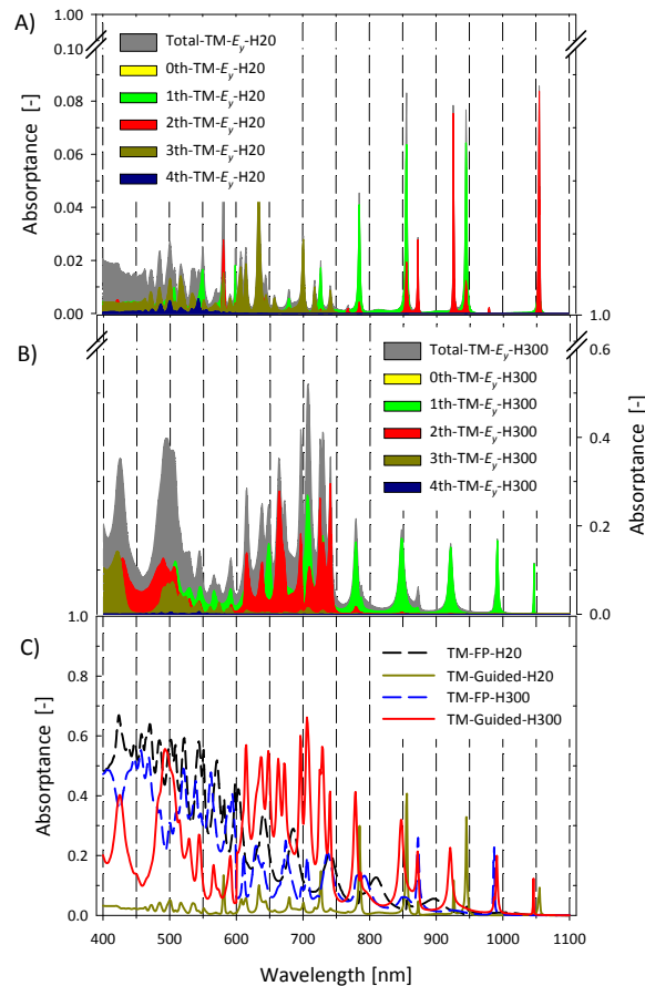
Fig. 8. (A)–(B) Contribution of each diffraction order, for the E_y component of the electric field, to total absorption. (C) Total FP (dashed lines) and guided resonance (continuous lines) triggered absorption, for shallow and large structure .
