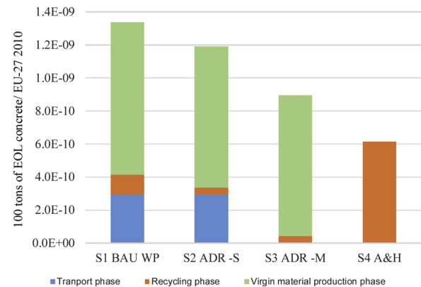
Fig. 8. Distribution of the weighted environmental impact score in three phases.
