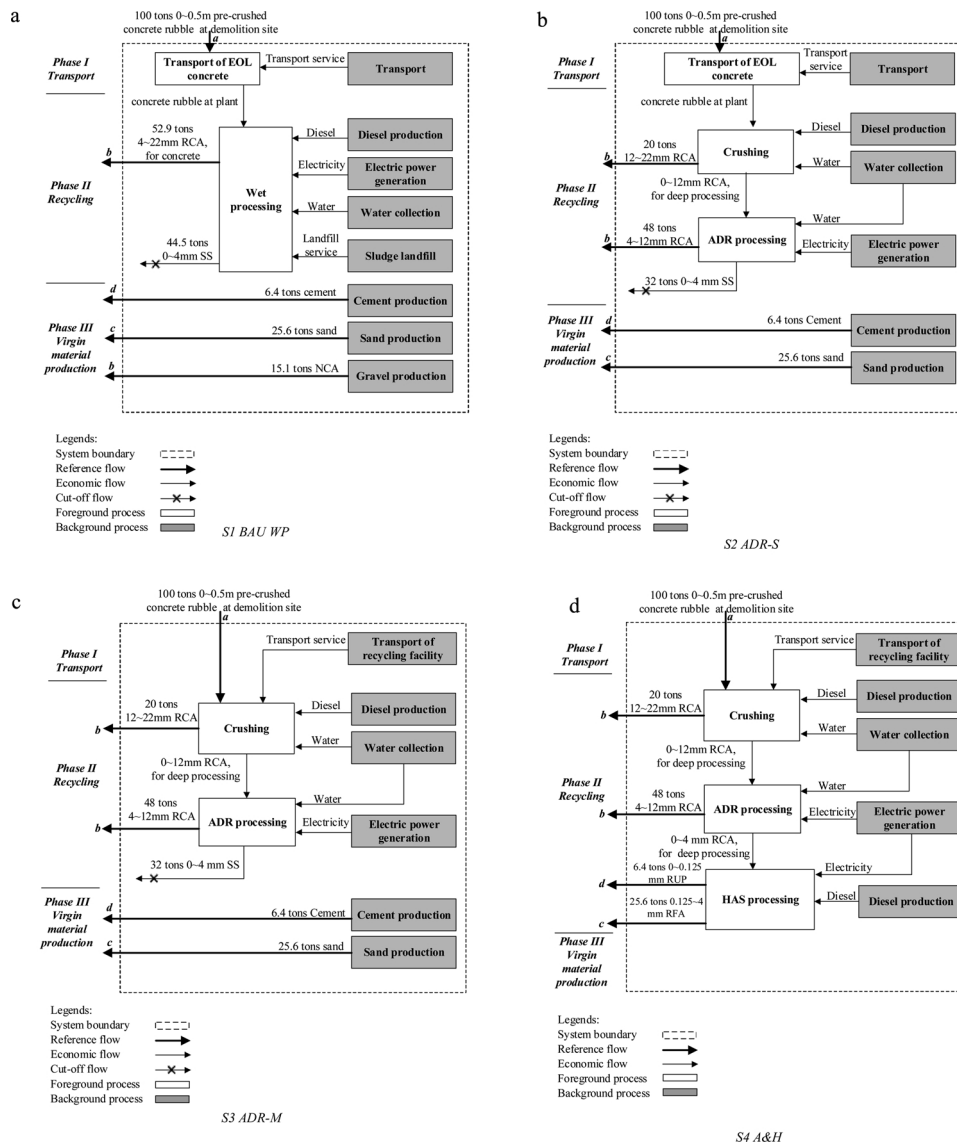
Fig. 5. Flow diagrams for the four systems: (i). S1 BAU WP (wet process) system; (ii). S2 ADR-S (stationary) system; (iii). S3 ADR-M (mobile) system; and (iv). S4 A&H (ADR & HAS) system, those flows which cross through the system boundary are functional flows, those lower-case letters at the end of the reference flow arrows refer to the sub-functional unit in Table 2.
