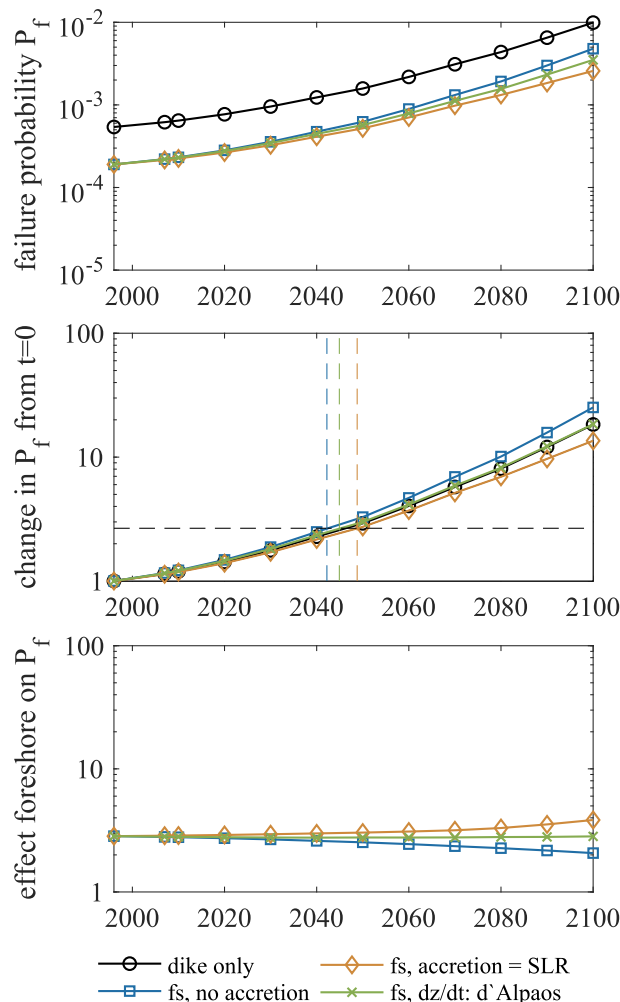
Fig. 10. Top panel: annual failure probability P_f in time for different accretion rates of the foreshore (abbreviation ‘fs’). Middle panel: the change in P_f with respect to t = 0 due to the combination of SLR and accretion (multiplication factor). Bottom panel: reduction factor of P_f with respect to the ‘dike only’ system.
