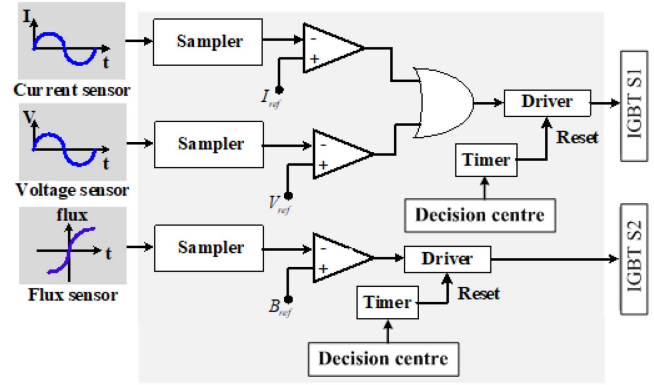
Fig. 6. Controller structure.
