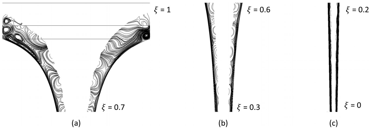
FIG. 9. Surface streamlines on the r - z sectional plane for the Twisted regime ( \dot{m}_{water,in} = 20.9 L/min).
