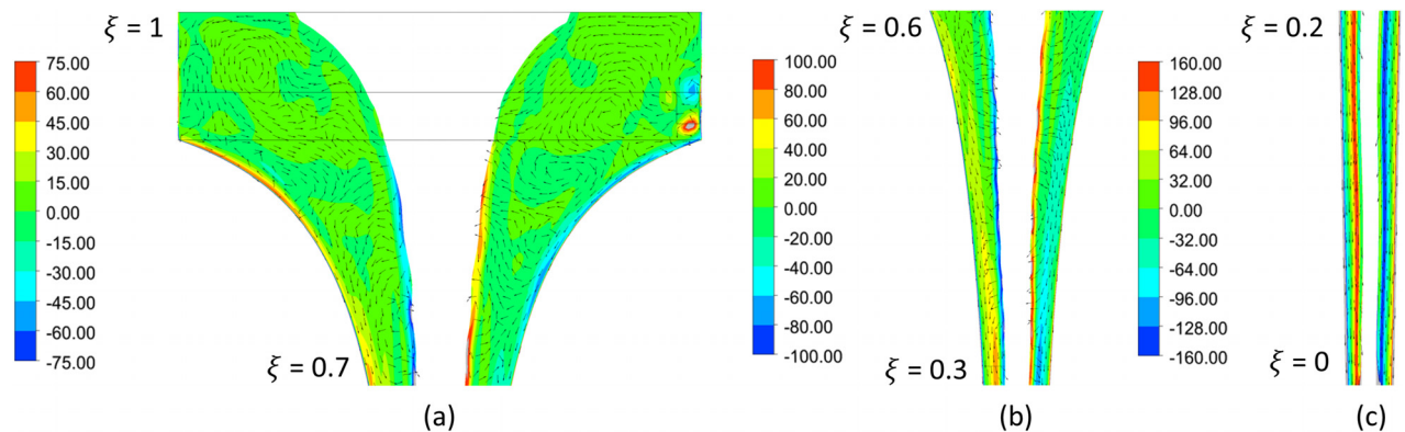
FIG. 16. Vorticity ( \Omega_\theta ) in r - z sectional plane for the Straight regime.
