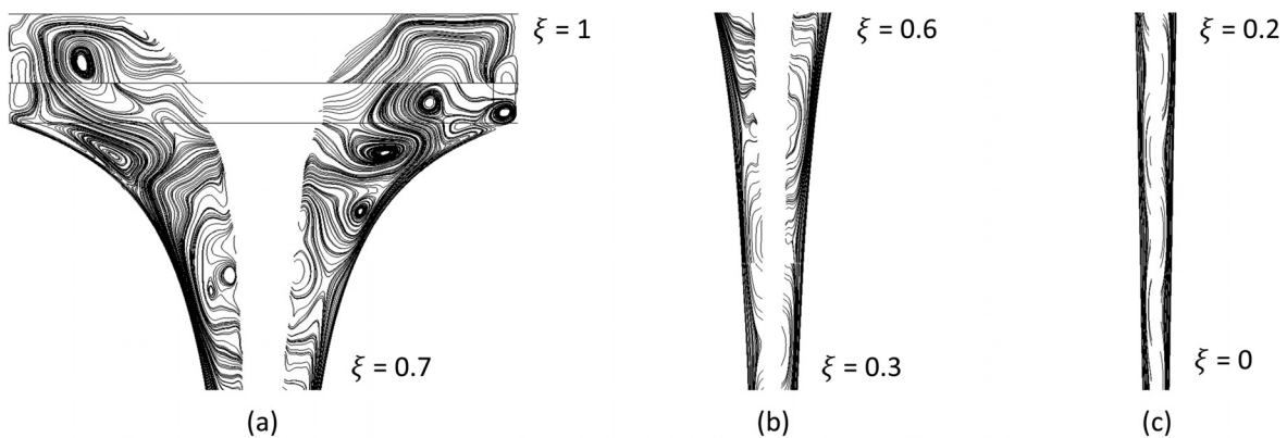
FIG. 10. Surface streamlines on the r - z sectional plane for the Straight regime ( \dot{m}_{water,in} = 22.5 L/min).
