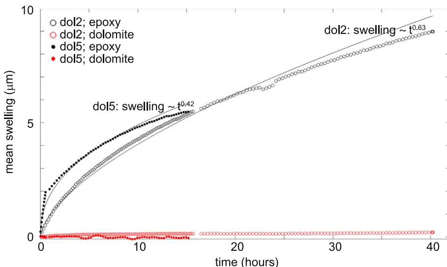
Fig. 5. Average swelling \delta z (μm) versus time for dol2 and dol5; epoxy in black and dolomite for reference in red. For dol5 there is a 3 bar pressure drop after the first hour (see Table 1), which changed the slope of the swelling curve. The power law fit of the epoxy swelling is shown in black, with the corresponding time exponents. (For interpretation of the references to color in this figure legend, the reader is referred to the web version of this article.)
