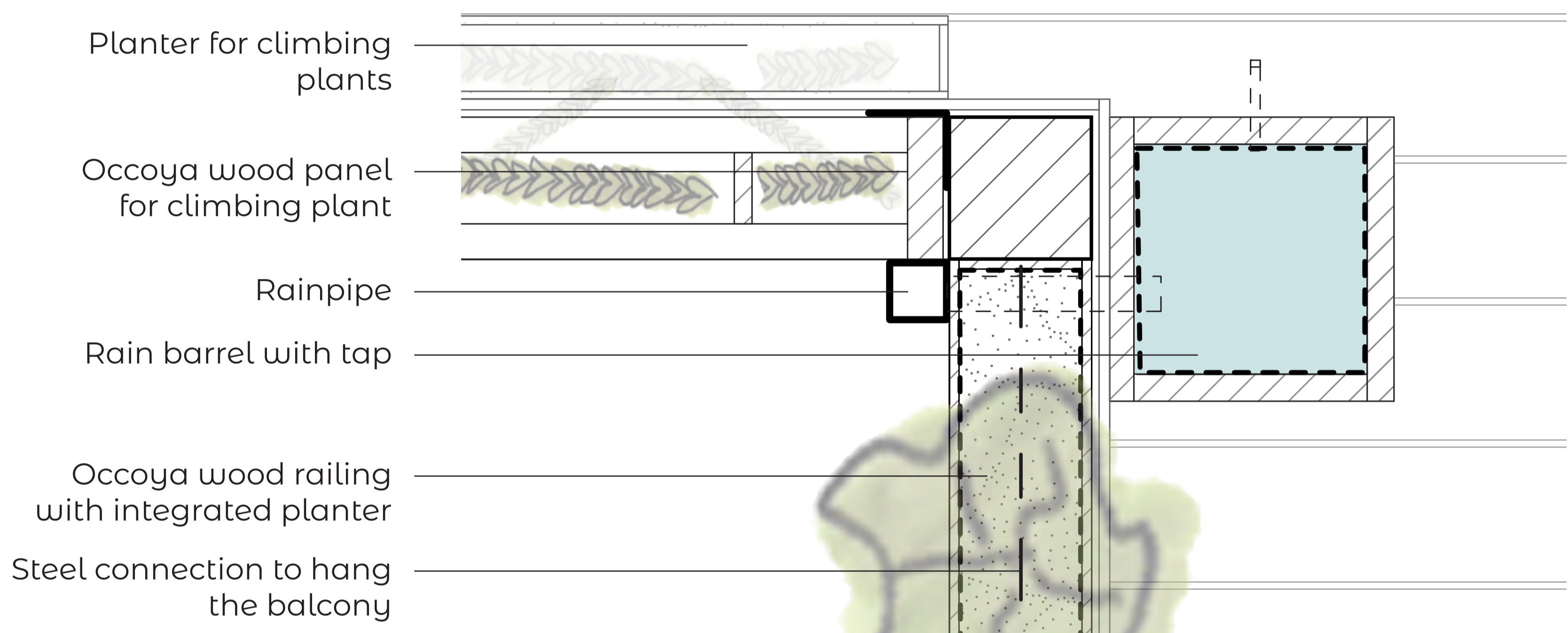
Detail gallery horizontal 1:5
