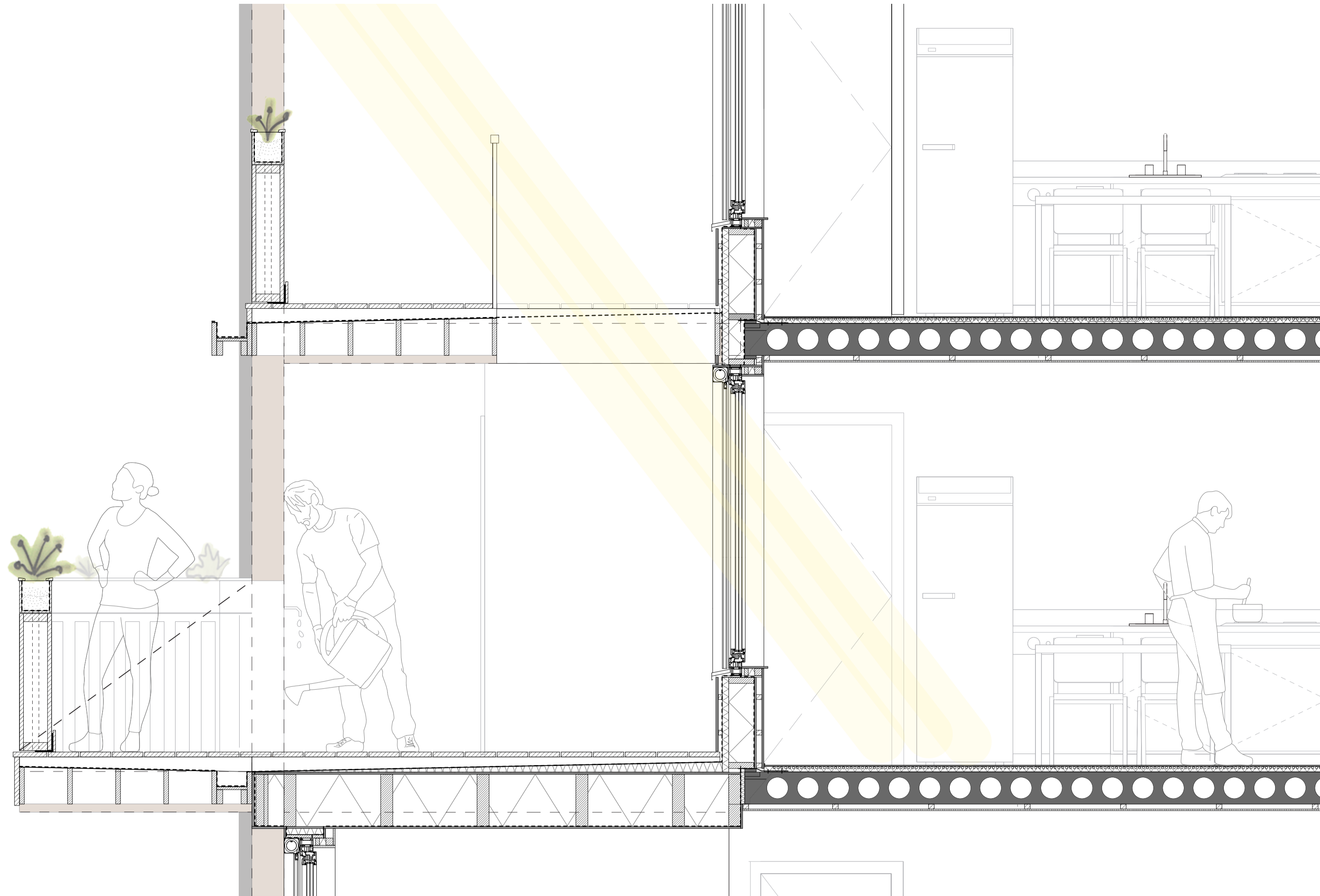
Facade fragment East 1:20
