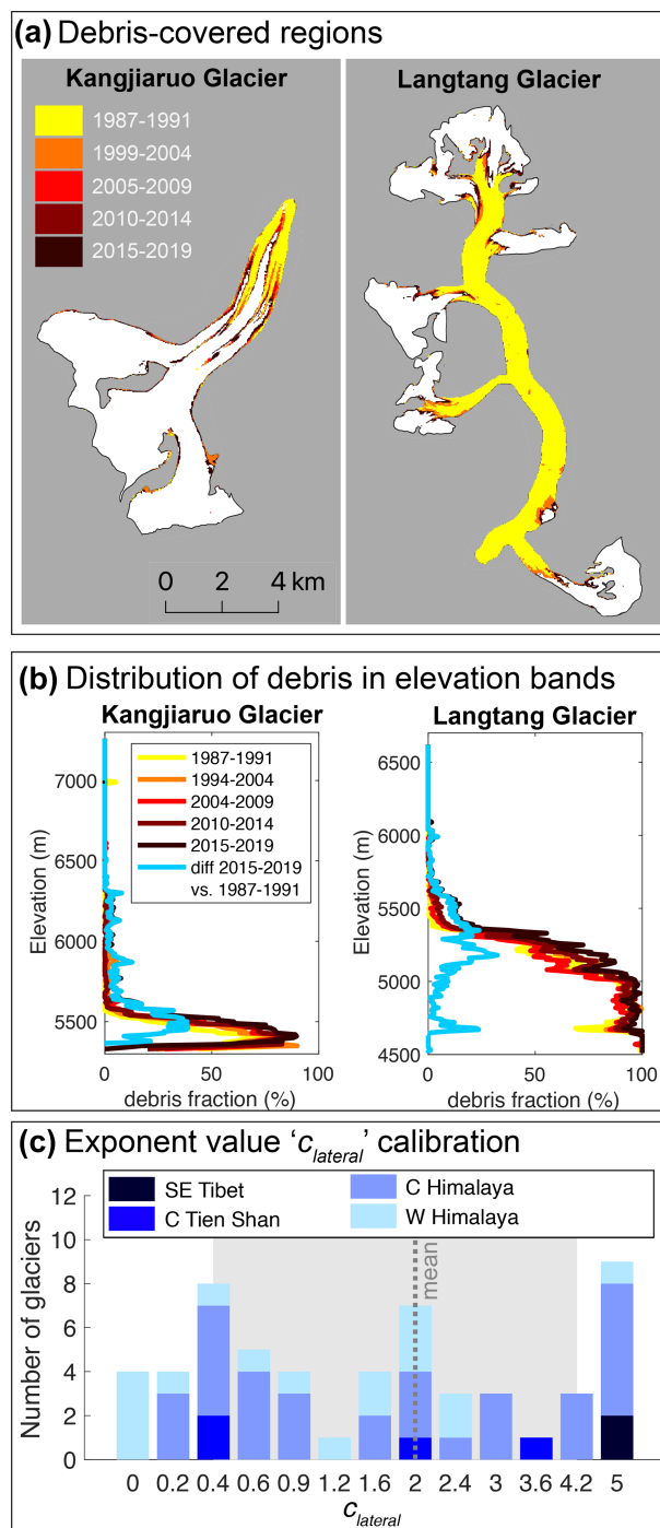
Figure 5. (a) Evolution of the debris-covered area of Kangjiaruo Glacier and Langtang Glacier as inferred from five Landsat scenes. (b) Same as (a) but divided into 10 m elevation bands. The blue line shows the lateral expansion of the debris cover as observed between the oldest (1987–1991) and the newest (2015–2019) Landsat scene. (c) Distribution of c_{\text{lateral}} resulting in the lowest misfit between observed and modelled debris-fraction evolution (given per number of glaciers). The grey dashed line shows the mean value, while the grey rectangle shows values within the 0.25 and 0.75 quantiles.
