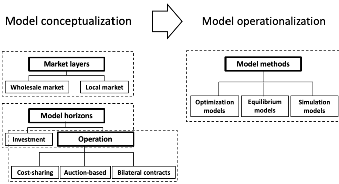
Fig. 1. Review framework.
