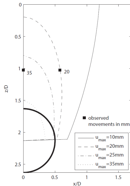
Fig. 12. Comparison of shallow tunnelling influence zones for the Barcelona Line 9 case
