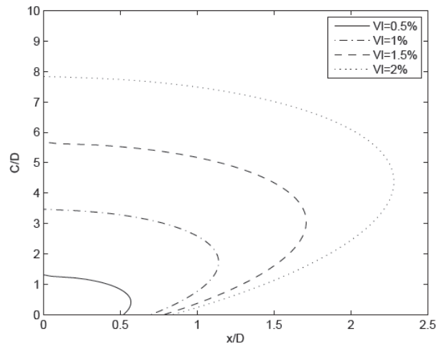
Fig. 4. Relationship between x/D and cover-to-depth C/D ratios in the case of tunnel with D = 6\text{m} in cohesive soil and the allowable settlement u_{\max} = 10\text{mm} (Vu et al., 2015a)
