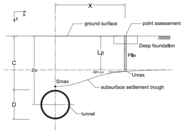
Fig. 5. Tunnel and exiting subsurface structures (Vu et al., 2015a)
