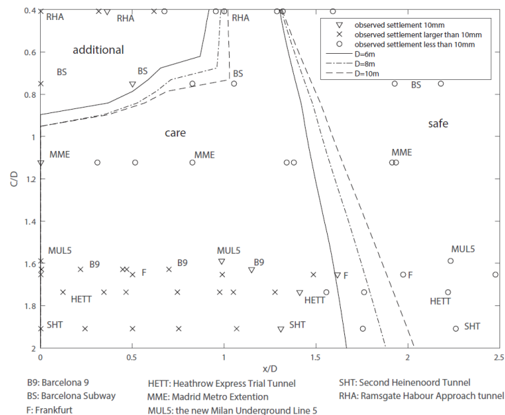
Fig. 10. Comparison of relative influence distances to shallow tunnelling cases
