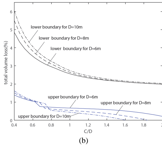
Fig. 2. Total volume loss for tunnelling in clay with various diameter D (Vu et al.,2015b)
