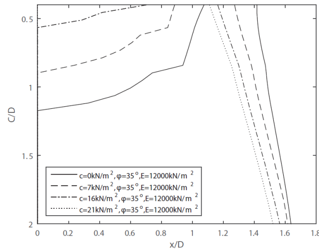
Fig. 13. Effect of cohesion c on relative influence distance x/D in the case of tunnelling with D = 6m
