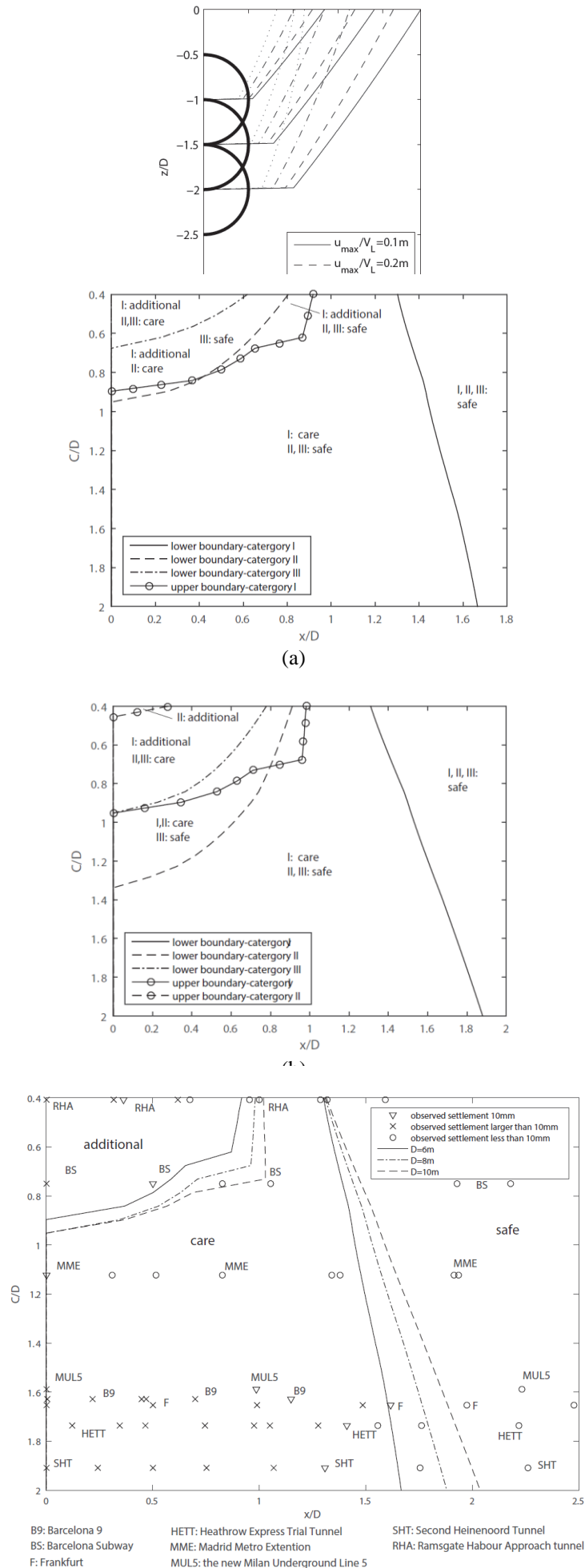
Fig. 10. Comparison of relative influence distances to shallow tunnelling cases
