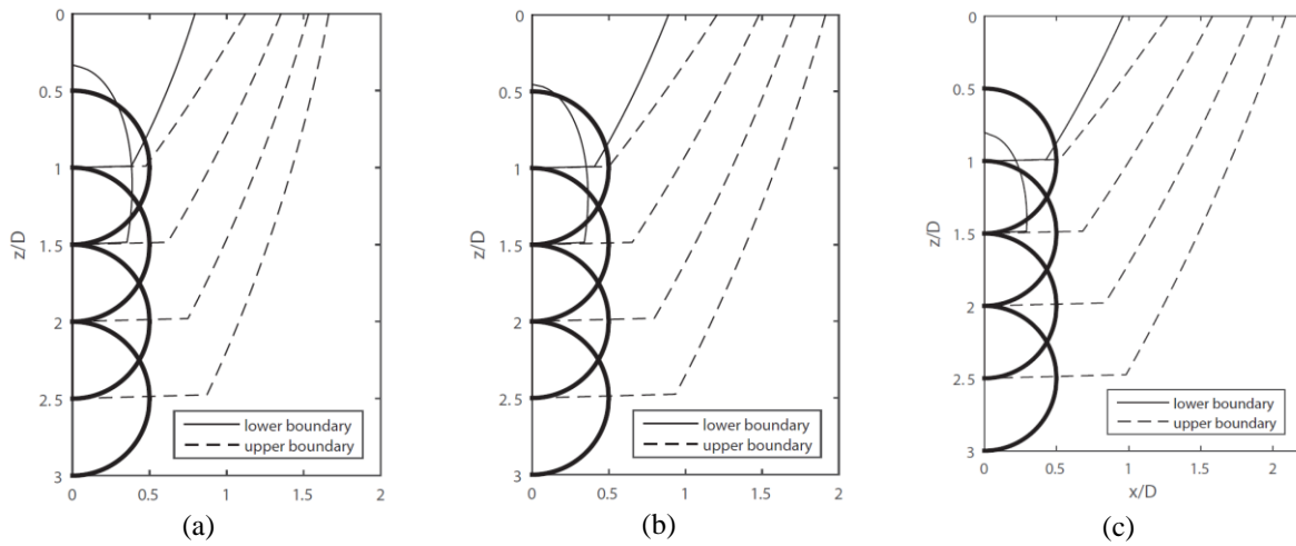
Fig. 11. Influence zones when shallow tunnelling in clay
