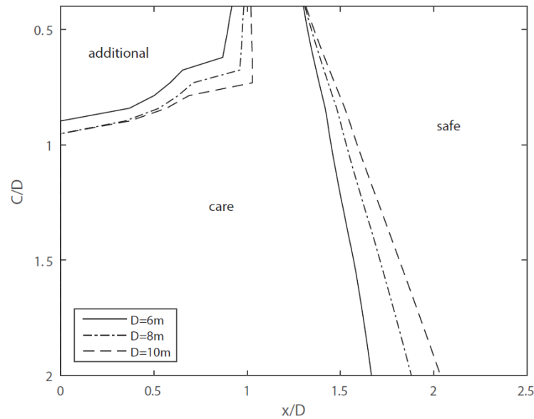
Fig. 9. Relative influence distances due to tunnelling in clay for risk category I with various tunnel diameter D
