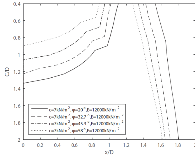
Fig. 14. Effect of friction angle \phi on relative influence distance x/D in the case of tunnelling with D = 6\text{m}
