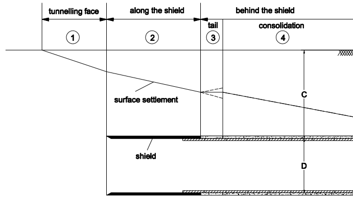
Fig. 1. Volume loss components (Vu et al., 2015b)
