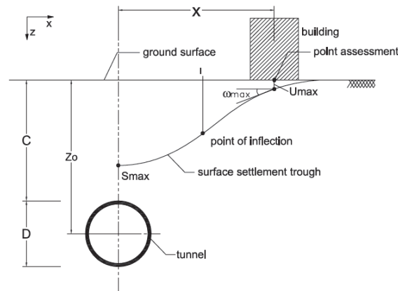
Fig. 3. Tunnel and existing surface building (Vu et al., 2015a)
