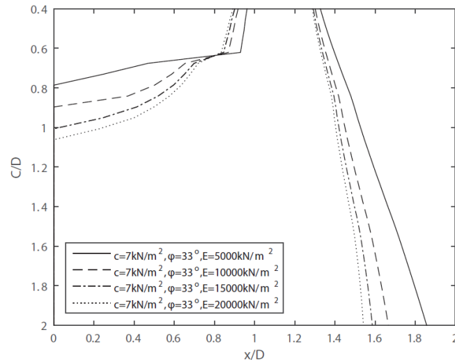
Fig. 16. Combination influence of soil parameters on relative influence distance x/D in the case of tunnelling with D = 6\text{m}
