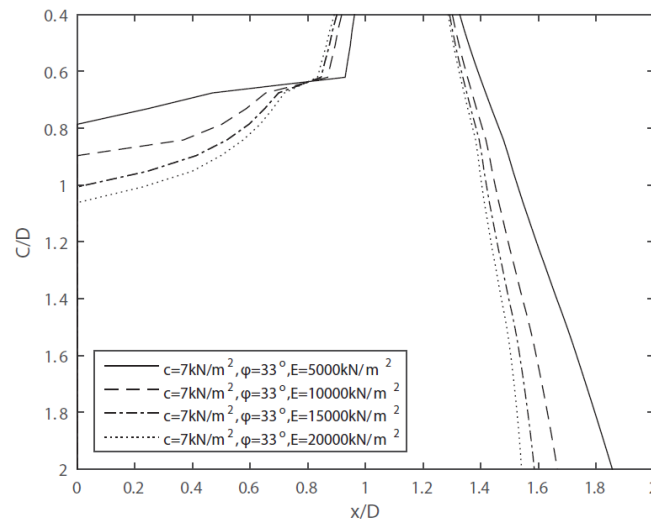
Fig. 15. Effect of modulus of elasticity E on relative influence distance x/D in the case of tunnelling with D = 6\text{m}
