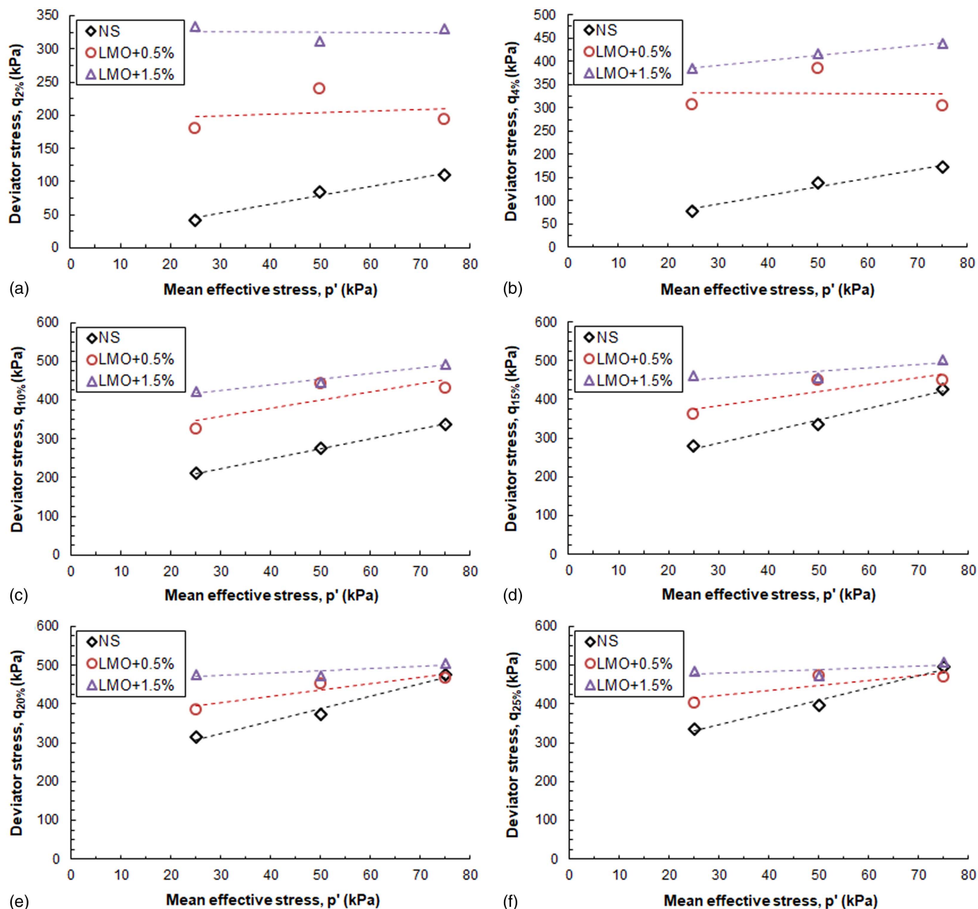
Fig. 12. Variation of deviator stress, q , at: (a) 2%; (b) 4%; (c) 10%; (d) 15%; (e) 20%; and (f) 25% axial strain with respect to initial mean effective stress, p'_i .
