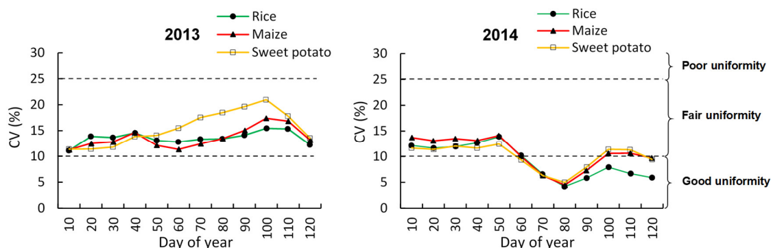
Figure 11. Variations of the uniformity of water consumption for paddy rice, maize, and sweet potato during January–April 2013 and 2014. The coefficient of variations (CV) of ET_a was used to characterize the uniformity of water consumption. Dashed lines represent the thresholds for distinguishing between irrigated areas with poor, fair, or good uniformity of water consumption.
