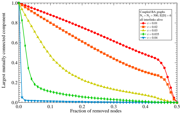
Figure 7.14: Largest mutually connected component as a function of the fraction of removed nodes in interdependent networks. The coupled graphs are Barabási-Albert with N = 500 and the average degree E[D] = 6 . The radius r in the random geometric graph is ranging from 0.01 to 0.04. The results are averaged over 10^3 realizations of interdependent graphs.
