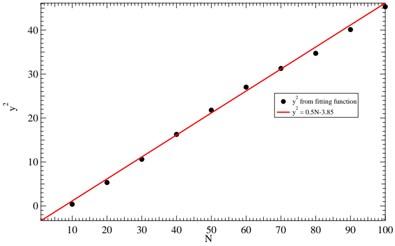
Figure 6.7: Fitting parameter y^2 = \frac{b}{a} as a function of N in ER graphs.
