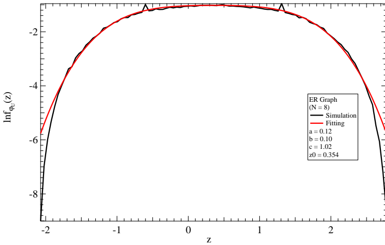
Figure 6.12: Natural logarithm \ln(f_{\phi_U}(z)) of the probability density function f_{\phi_U}(Z) for 10^8 ER graphs with p = 2\log(N)/N (to make sure the graph is connected) and N = 8 .
