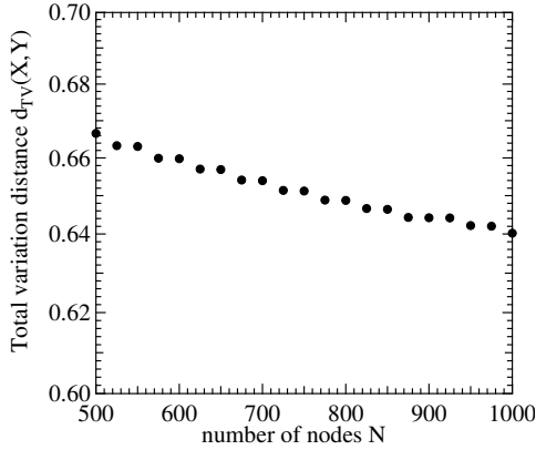
Figure 5.5: The total variation distance d_{TV}(X, Y) when the original graph has different number of nodes from 500 to 1000.
