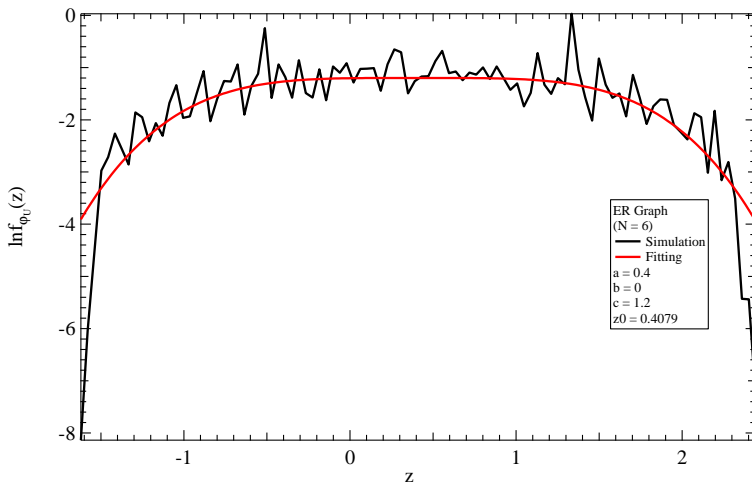
Figure 6.13: Natural logarithm \ln(f_{\phi_U}(z)) of the probability density function f_{\phi_U}(Z) for 10^8 ER graphs with p = 2\log(N)/N (to make sure the graph is connected) and N = 6 .
