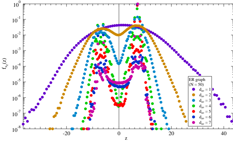
Figure 6.1: The probability density function of s_Z in ER random graphs G_p(N) for N = 50 and various average degree d_{av} = p(N - 1) , ranging from d_{av} = 1 up to d_{av} = 7 . The y-axis is in log-scale.
