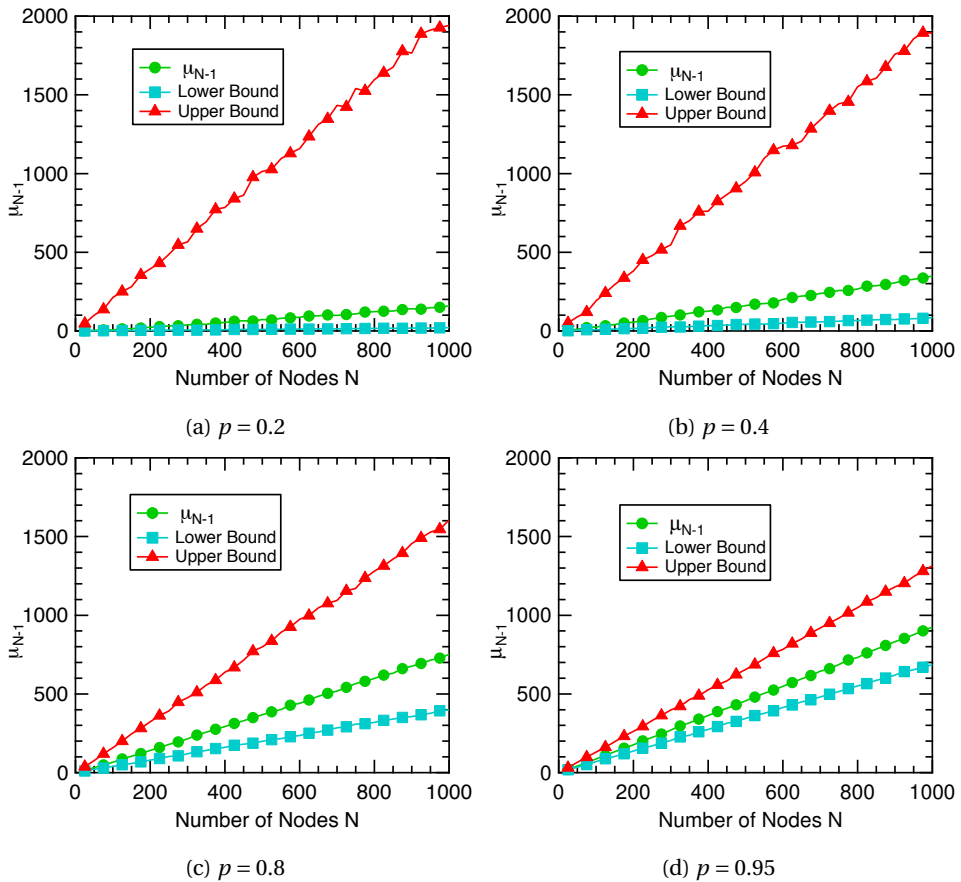
Figure A.1: Upper and lower bounds of the algebraic connectivity \alpha_G .
