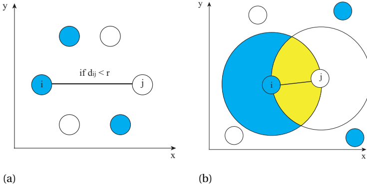
Figure 7.1: Two topologies for B : (a) random geometric graph; (b) relative neighbourhood graph: since there is no third node in the intersection region (marked as yellow), nodes i and j are connected. Nodes from G_1 are represented with filled circles, whereas nodes from G_2 are represented with unfilled circles.
