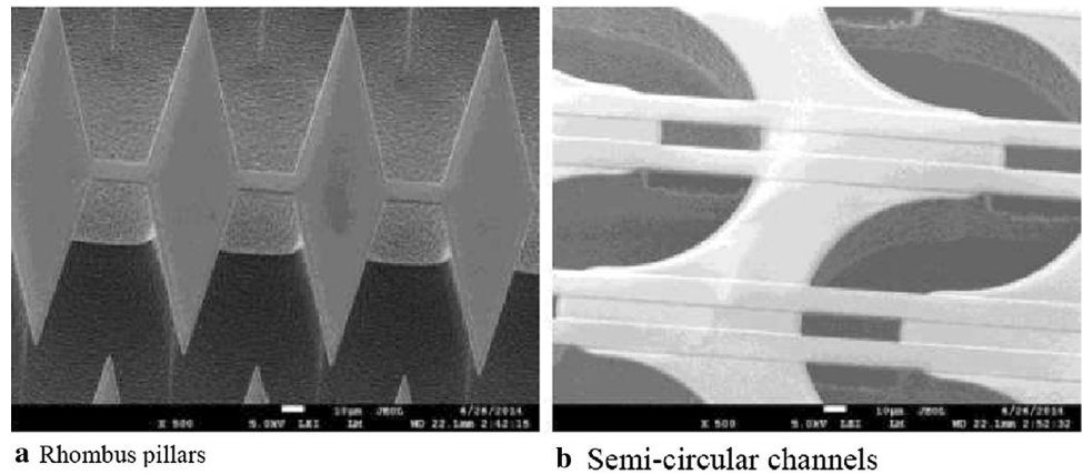
Fig. 3 SEM pictures of the suspended heating elements for two different geometries [13]
