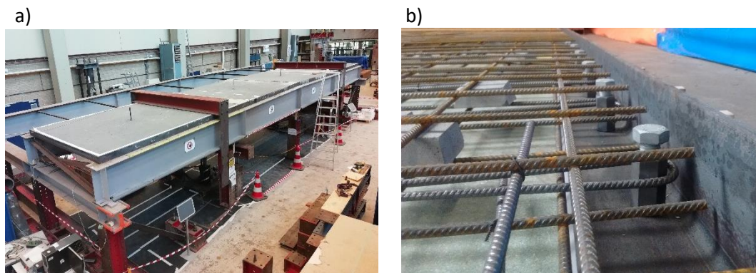
Figure 3 - a) Experimental set-up, b) Prefabricated deck prior to casting, indicating the reinforcement and embedded couplers and bolts.
