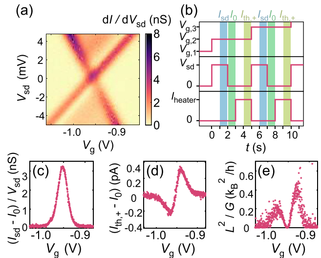
FIG. 3. (a) Differential conductance dI/dV_{\text{sd}} as a function of applied gate V_g and bias V_{\text{sd}} voltages. (b) Measurement scheme used to measure I_{\text{th}}(V_g) and G(V_g) as a function of gate voltage. The shaded regions indicate the time windows in which current measurements are performed. (c) Conductance, (d) I_{\text{th}} and (e) power factor as a function of V_g .
