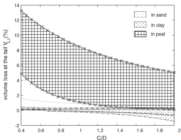
Figure 9. Volume loss at the tail in various soil when tunnelling with D=6 m
