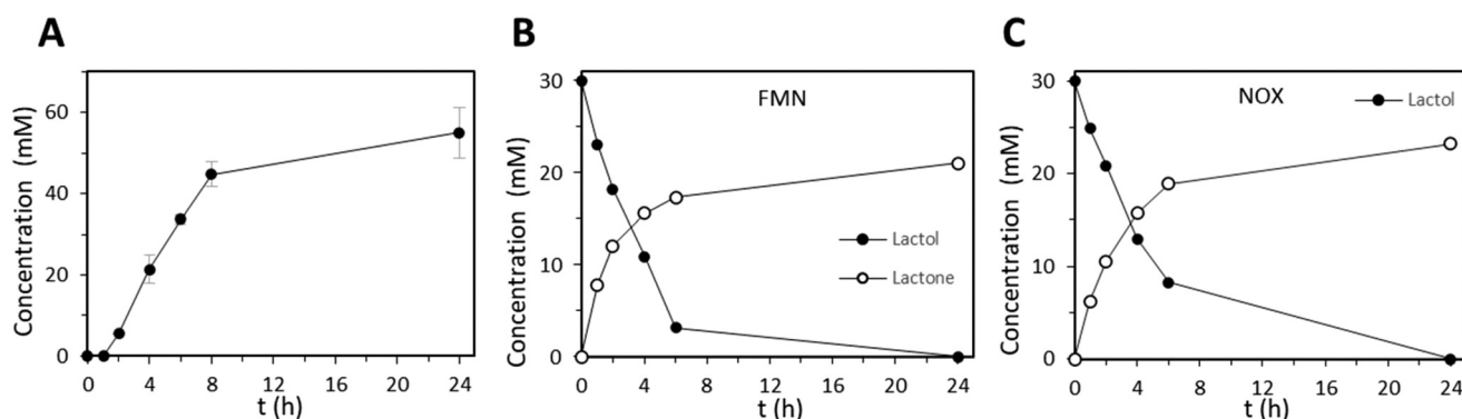
Fig. 6 Enzymatic cascade for the production of lactone 4 . A . Fed batch synthesis of lactol 3 (●) catalysed by DERA. 1 U mL -1 of purified Lb DERA C42M E78K in 45 mL 100 mM TEA pH 7.0 buffer, room temperature, stirring, under nitrogen. 3 M of acetaldehyde in 100 mM TEA pH 7.0 buffer fed with flowrate 0.5 mL h -1 to an end concentration of 300 mM and end volume of 50 mL. 500 μL of samples were taken in duplicates over time and analysed with GC. B . Oxidation of lactol 3 (●) to lactone 4 (○) catalysed by ADH440 with FMN regeneration system. The reaction mixture of A was mixed with ADH440, NADP + , FMN, and catalase. The final concentrations in the reaction were: 30 mM lactol, 40 U mL -1 ADH440, 5 mM NADP + , 1 mM FMN, and 60 U of catalase in 20 mL TEA pH 7.0 buffer in a 100 mL round bottom flask. The reaction mixture was exposed to blue light (465 nm), 30 °C, and stirred. 200 μL samples were taken over time and analysed with GC. C . Oxidation of lactol 3 (●) to lactone (○) catalysed by ADH440 with NOX as regeneration system. The reaction mixture of A was mixed with ADH440, NADP + , and NOX. The final concentrations in the reaction were: 30 mM lactol, 40 U mL -1 ADH440, 5 mM NADP + , and 5 mg mL -1 NOX in 20 mL 100 mM TEA pH 7.0 buffer in a 100 mL round bottom flask. The reaction mixture was heated to 30 °C, and stirred. 200 μL samples were taken over time and analysed with GC.
