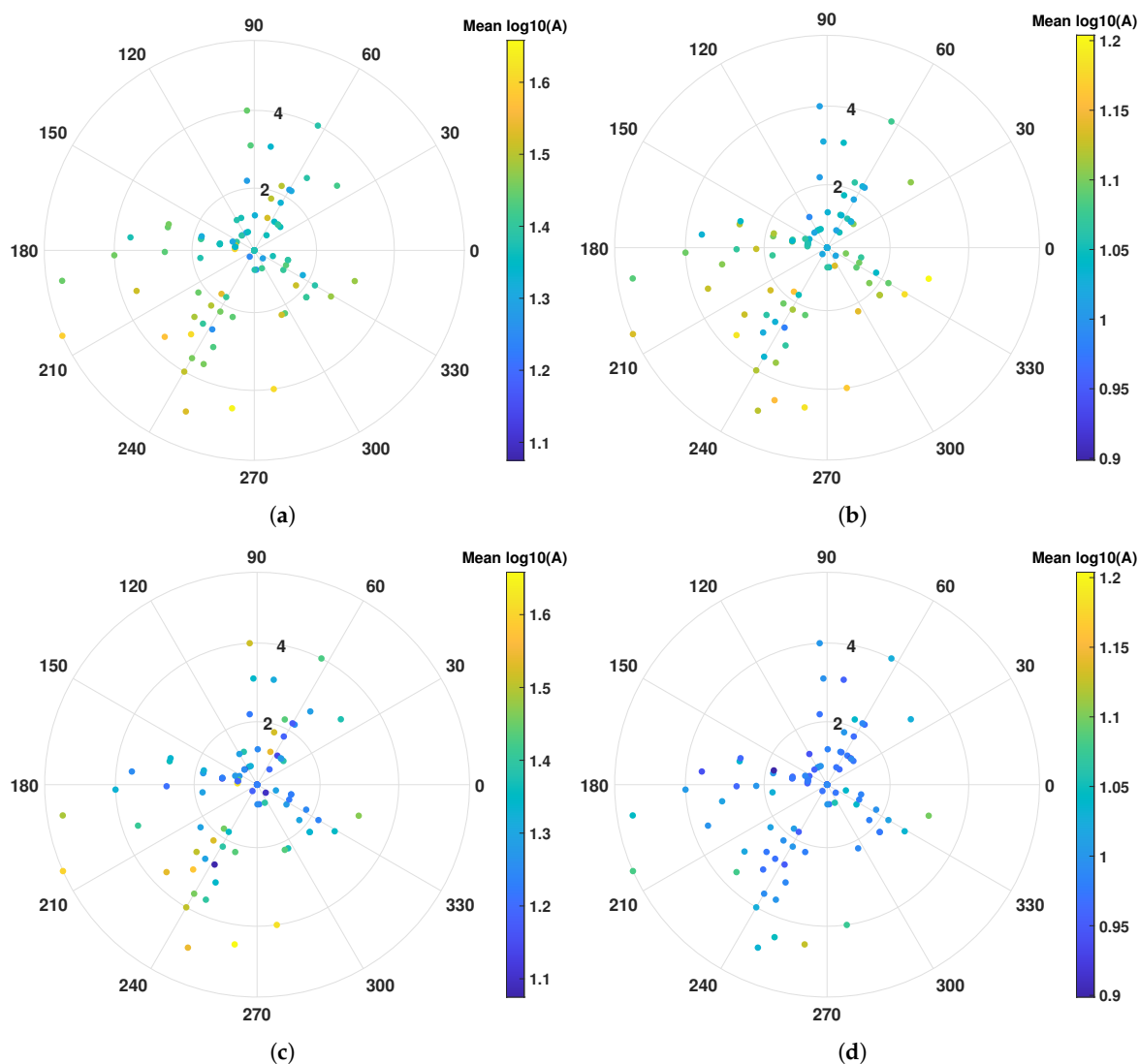
Figure 9. Amplitude in logarithmic scale (color bar) as a function of the wind direction ( 0^\circ = \text{North} ; 90^\circ = \text{East} ) and wind intensity (m/s; represented on the radius). Amplitude in VV and VH polarizations is represented, respectively, on the sand mask in the panels (a,b), and on the sea mask in the panels (c,d). A dependence of amplitude on the wind direction can be noticed both in the two masks and in the two polarization. In general, for both polarizations and both masks, high wind intensity is associated with high amplitude values. For some wind angle (i.e., 210^\circ\text{--}240^\circ ), the dependence of the amplitude on the wind is more considerable.
