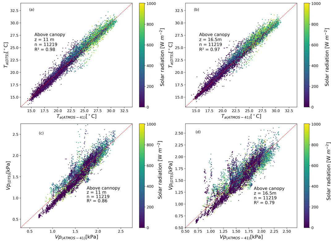
Figure 5. Comparison of DTS temperature ( T_{a(\text{DTS})} ) and actual vapour ( VP_{(\text{DTS})} ) measurements with the ATMOs-41 ( T_{a(\text{ATMOs-41})} and VP_{(\text{ATMOs-41})} ) measurements at 11 and 16.5 m above the forest canopy.
