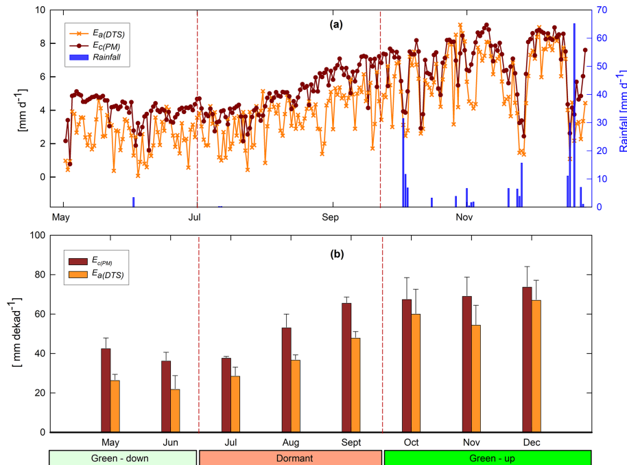
Figure 8. (a) May–December 2021 daily (06:00–18:00 LT) estimates of evaporation E_{a(DTS)} using the BR-DTS and E_{c(PM)} using the PM. (b) Comparison of dekadal evaporation estimates between E_{a(DTS)} estimates and E_{c(PM)} ( E_c = K_c E_o ). The E_{a(DTS)} and E_{c(PM)} show good agreement in both dry and rainy seasons and across canopy phenophases. Overall, at dekadal scale, the E_{c(PM)} is relatively higher than E_{a(DTS)} (b). Phenophases classification: May–June is the green-down phenophase, July–September is the dormant phenophase, and October–December is the green-up phenophase.
