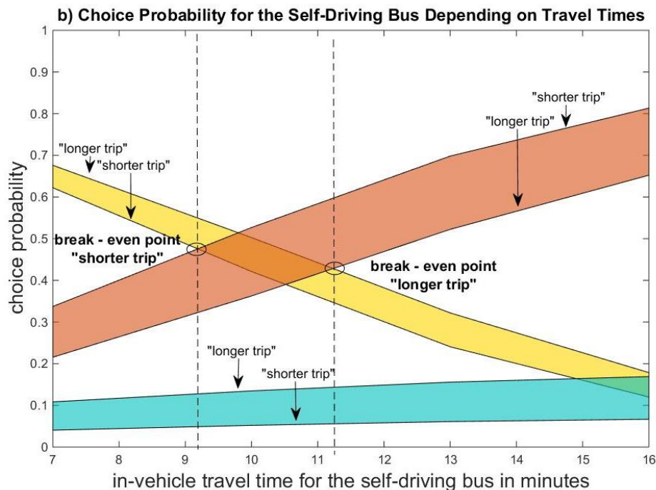
Figure 2.1: Choice probabilities for the automated bus (yellow), regular bus (red) and other alternatives (turquoise) for different (a) travel fares and (b) travel times for the self-driving bus for two scenarios. The break-even points are marked by a dotted line.
