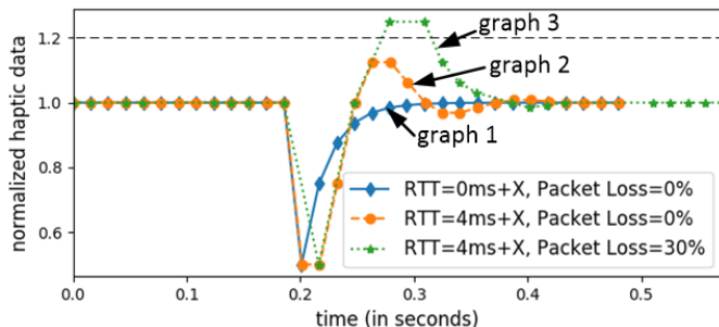
Fig. 16. Step response for different RTT and packet drop percentages. X represents the component of RTT that is not part of emulation. The change in pressure ( 1 \rightarrow 0.5 ) occurs at \approx 0.2 s.
