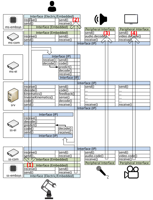
Fig. 3. APIs in the forward and backward flow paths in a TCPS. (1) represents the kinematic flow. (2), (3), and (4) represent the haptic, audio, and video flows respectively.
