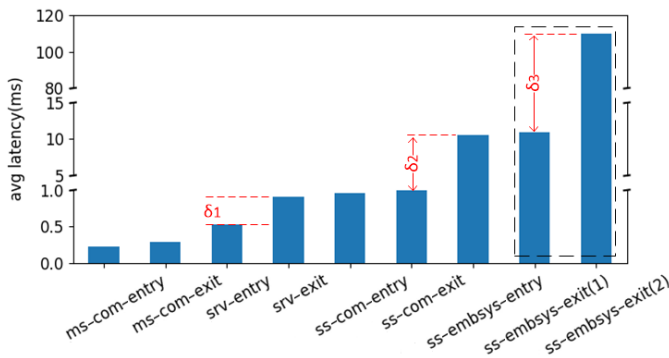
Fig. 8. Average latencies measured for different echo points. For all the latency bars, the margin of error is within 5%.
