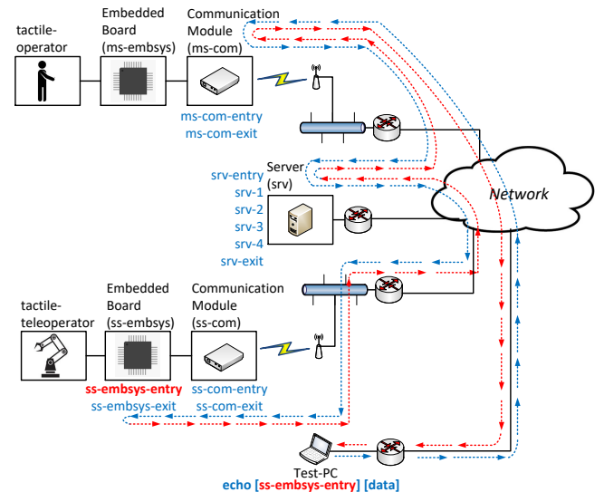
Fig. 4. In-situ latency test. The path taken by the echo command targeting echo point ss-embsys-entry is marked. Only the echo points in the forward kinematic data path are shown.
