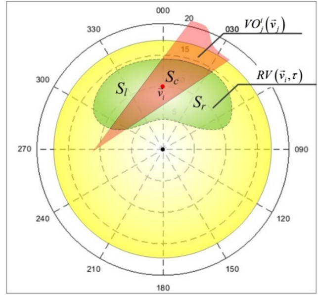
Fig. 2. Illustration of the dangerous set and the reachable set in the velocity space of the OS. (note: a point in this space represents a velocity of the OS: the axes indicate the course; the distance from the pole represents the speed).
