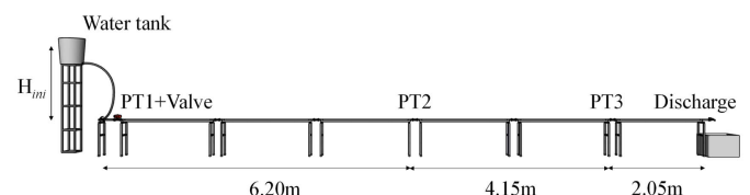
Fig. 1. Schematic representation of the pipe-rig layout.
