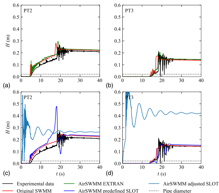
Fig. 8. Experimental data versus numerical results for H_{ini} = 0.35 m and large orifice configuration: (a and b) with the EXTRAN model at PT2 and PT3; and (c and d) with SLOTT method with SWMM predefined slot width and with the adjusted slot width at PT2 and PT3.
