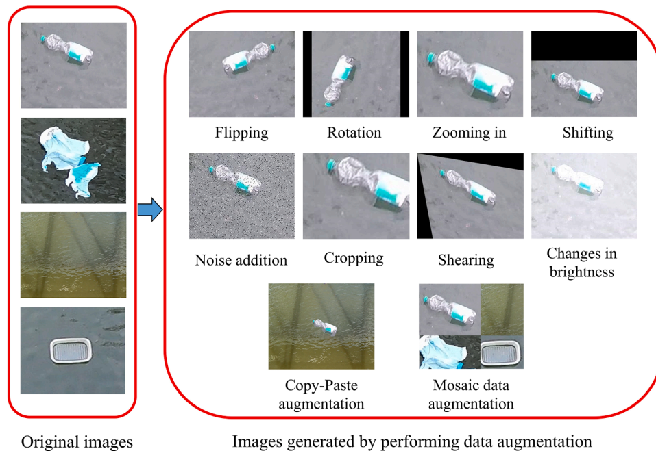
Fig. 5. Examples of data augmentation techniques used in reviewed papers to improve model performances. Left: original images; Right: images generated by performing geometrical transformations (e.g., flipping, rotation, zooming in, shifting, cropping, and shearing), and other basic (e.g., changes in brightness, and noise addition), or advanced transformations (e.g., copy-paste augmentation, and mosaic data augmentation).
