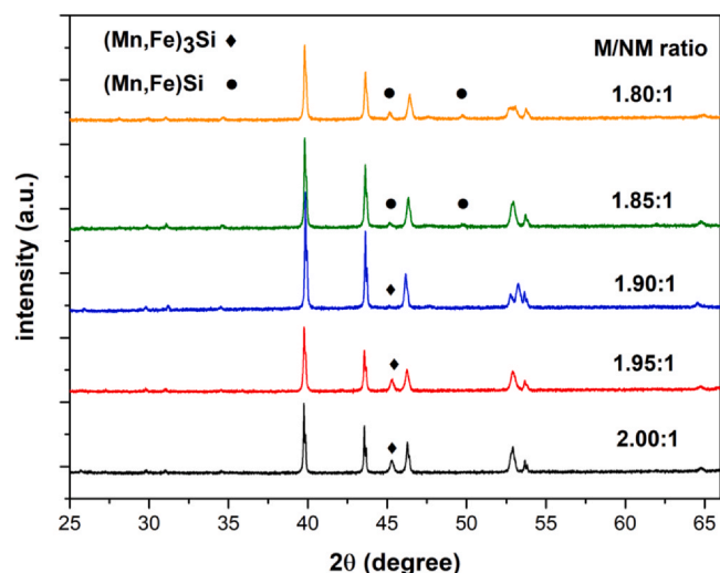
Fig. 1. XRD patterns measured for the (\text{Mn,Fe})_y(\text{P,Si}) alloys annealed at 1373 K ( y = 1.80, 1.85, 1.90, 1.95, 2.00 ).
