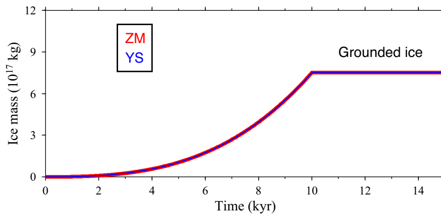
Figure 8. Time evolution of grounded ice for benchmark C.
