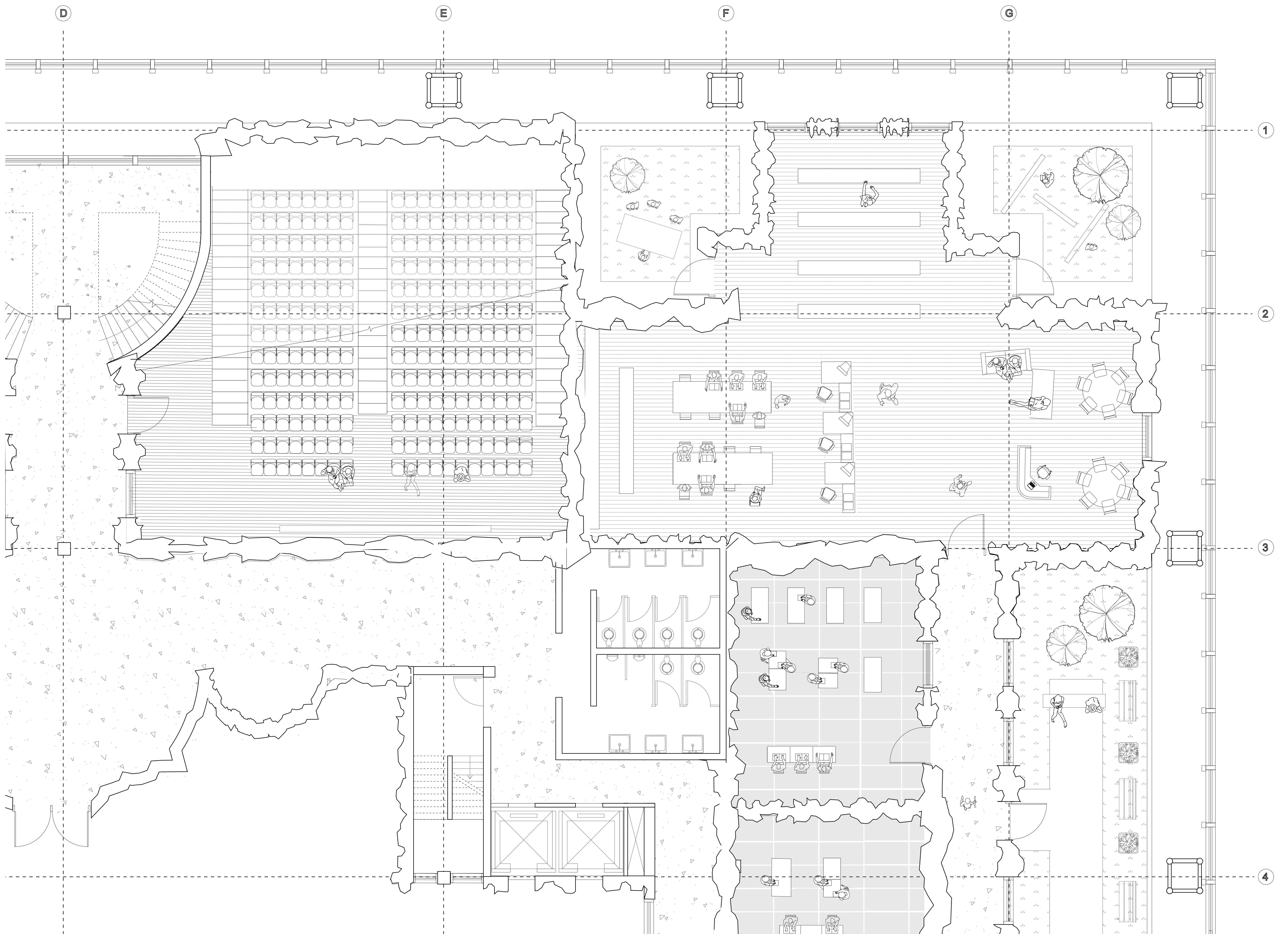
First Floor Fragment Plan
