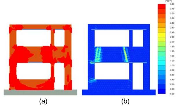
Figure 8. Plastic points (red coloured areas) (a) and total deviatoric strains (b) in the superstructure.
