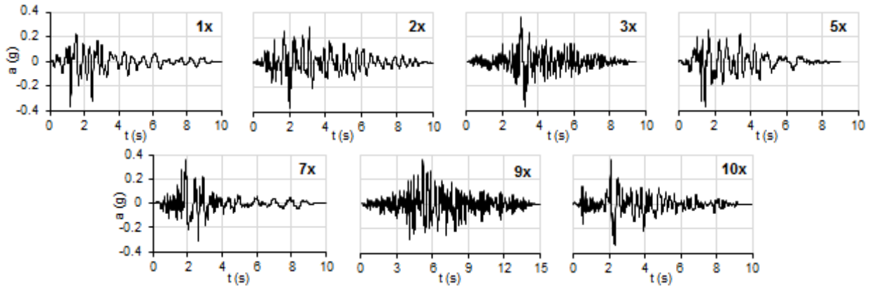
Figure 3. Selected input time histories from the database of NPR 9998:2015, linearly scaled to a PGA of 0.36 g.
