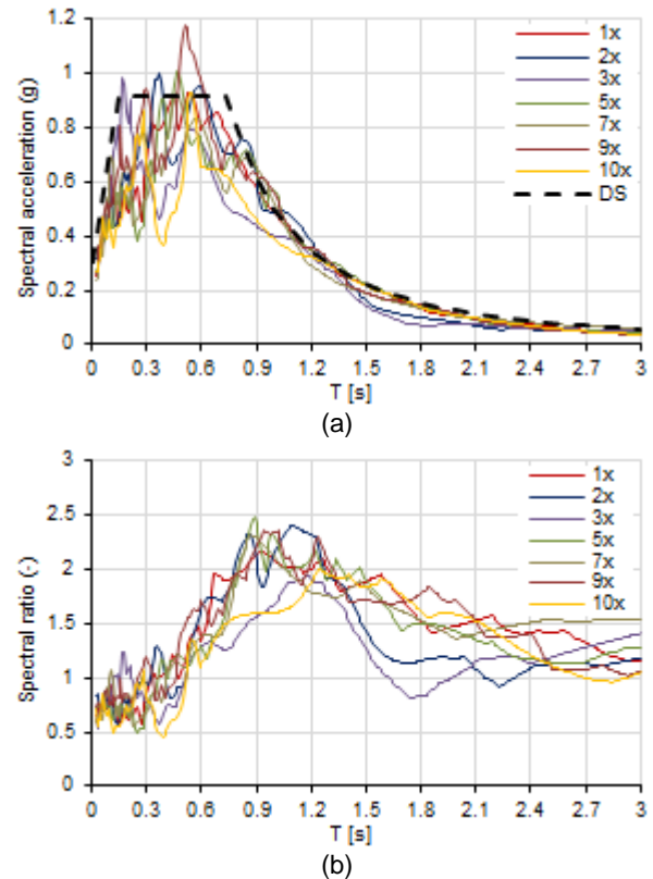
Figure 5. Spectral acceleration at ground surface for seven input time histories with PGA equal to 0.36 g and structural damping ratio \xi=5\% (a) and spectral ratio between input (half-space) and output (ground surface) spectral acceleration spectra.
