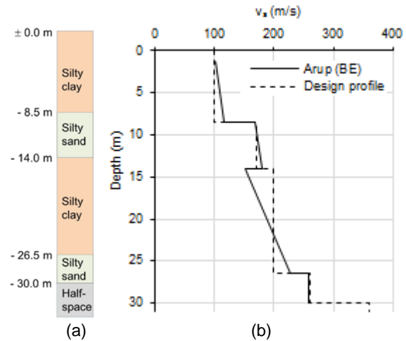
Figure 1. Soil stratigraphy (a) and best estimate (BE) shear wave velocity profile provided by Arup (2015), and selected design profile for the present study (b).
