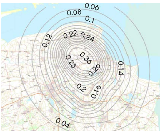
Figure 4. Hazard map of Groningen indicating the maximum expected PGA values at ground level for a 475-year return period (NPR 9998:2015).
