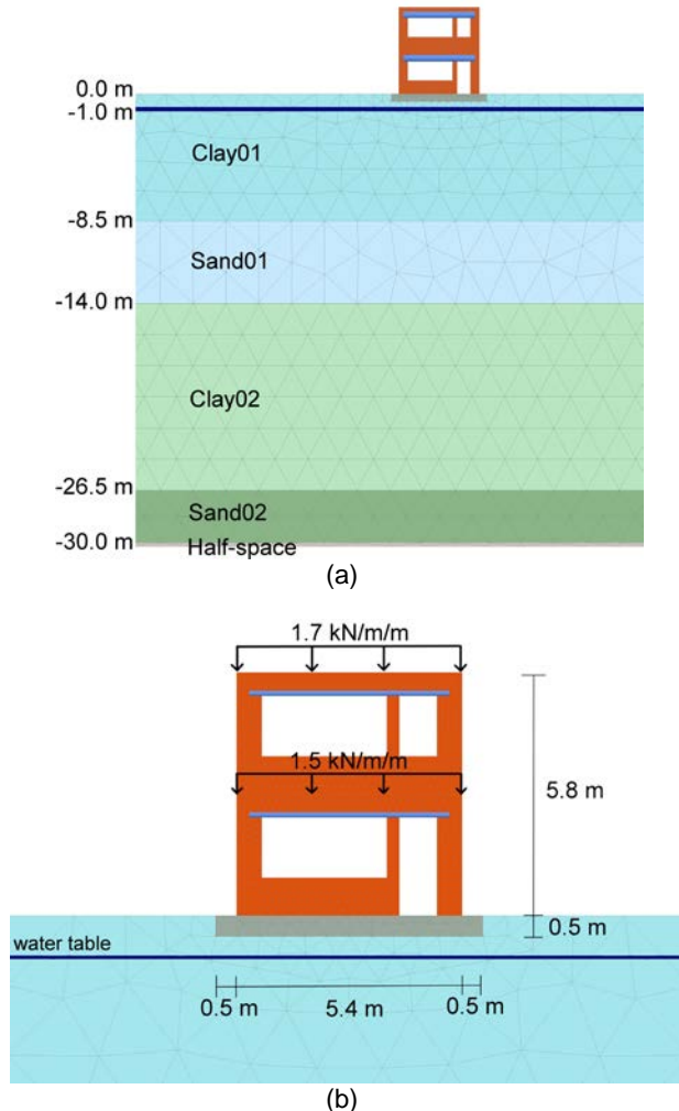
Figure 6. Model geometry and finite element mesh for the case study (a) and close-up of the superstructure (b).
