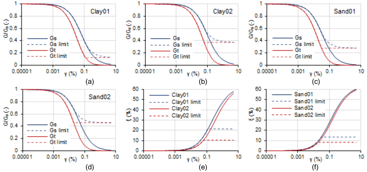
Figure 2. Shear stiffness degradation curves for Clay01 (a), Clay02 (b), Sand01 (c) and Sand02 (d), and the corresponding damping ratio curves for clay (e) and sand (f) profiles.
