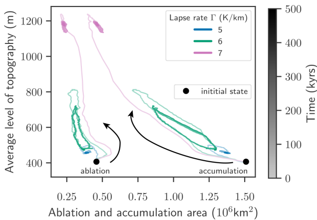
Figure 7. State space trajectories for different regimes for the three different lapse rates \Gamma = [5, 6, 7] K km^{-1} . The curves represent the average height of the bedrock topography vs. the ablation and the accumulation area. Blue: lapse rate \Gamma = 5 K km^{-1} , incomplete recovery of the ice volume. Green: lapse rate \Gamma = 6 K km^{-1} , oscillation of the ice volume. Purple: lapse rate \Gamma = 7 K km^{-1} , irreversible loss of the ice volume. The color code corresponds to Fig. 2 a; that is the temperature forcing is \Delta T = 2 K and the mantle viscosity is \eta = 1 \times 10^{21} Pa s . The color shading represents time, as indicated by the color bar on the right side. The average bedrock and the accumulation and ablation area of the initial state are represented by the black marker.
