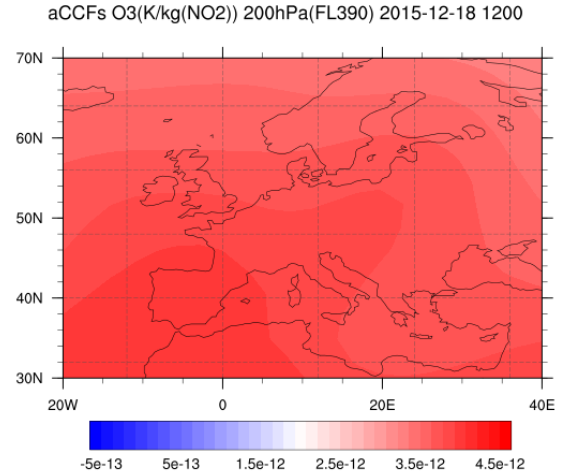
Fig. 2: The temperature response ( \text{K}/\text{kg}(\text{NO}_2) ) calculated by the ozone aCCFs on a specific day 1200 hour at 200 hPa.
