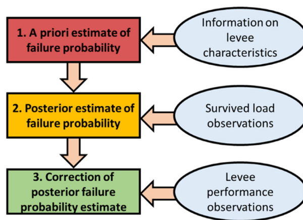
FIGURE 4 Schematization of the proposed method to estimate the failure probability, utilizing information on levee performance under critical conditions and levee inspection results
