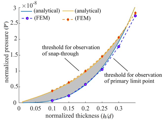
Fig. 11. The pressure range in order to trigger the primary limit point and the snap-through, as a function of thickness of the flexible electrode, with R = 100 \mu\text{m} .
