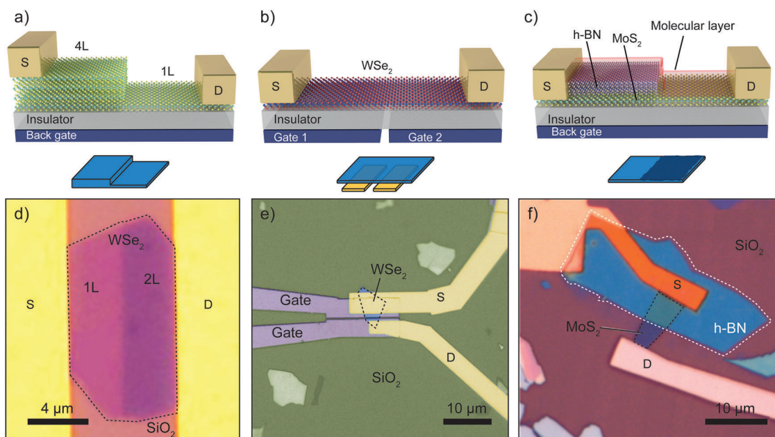
Fig. 4 Different examples of p–n junctions based on 2D materials homojunctions. (a–c) Schematic diagram of a p–n junction based on (a) MoS 2 with different thickness, (b) ambipolar WSe 2 with two split gate electrodes and (c) local molecular doping of partially h-BN encapsulated MoS 2 . (d) Optical image of a thickness-modulated p–n junction based on single-layer and bilayer WSe 2 . (e) Optical image of a split-gate homojunction as schematically drawn in panel (b). (f) Optical image of a chemically doped MoS 2 p–n junction as schematically illustrated in panel (c). The device is covered with molecules and part of the MoS 2 is protected by a h-BN flake. Panel (d) readapted from ref. 73 with permission from IOP Publishing, panel (e) readapted from ref. 77 with permission from Springer Nature and panel (f) readapted from ref. 88 with permission from American Chemical Society (copyright 2014).
