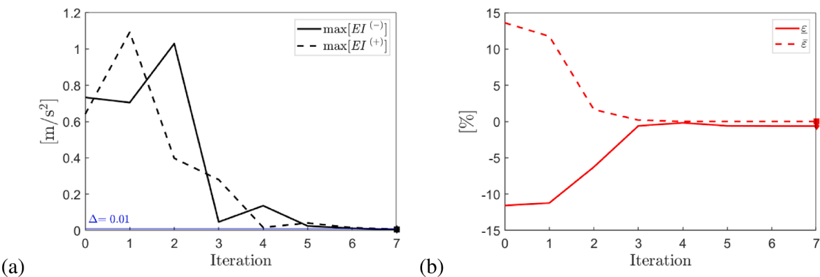
Fig. 11. Approach B results for each iteration expressed in terms of: (a) \max[EI^{(-)}] (solid line) and \max[EI^{(+)} (dashed line); (b) percentage errors \epsilon (solid line) and \bar{\epsilon} (dashed line). The constant blue line corresponds to the tolerance value \Delta . (For interpretation of the references to colour in this figure legend, the reader is referred to the web version of this article.)
