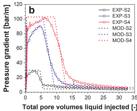
Fig. 3. Comparison of sectional pressure gradients in core-flood experiments with those obtained from the linear bank-propagation model during liquid injection following about 150 PV gas injection at various superficial velocities. (a) 2 ft/day, (b) 20 ft/day, (c) 80 ft/day, and (d) 200 ft/day. EXP: experimental data. MOD: model fit. S2, S3, S4: Sections 2–4.
