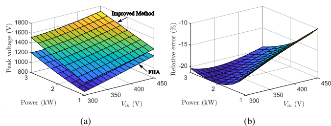
Fig. 15: S-S compensation. (a) Peak voltage of secondary coil. (b) Relative error.
