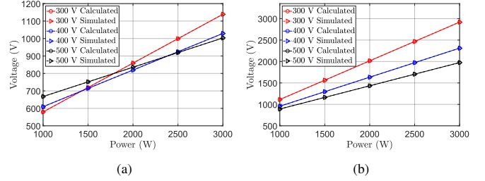
Fig. 7: LCC-S compensation, M = 70 \mu\text{H} . (a) Peak voltage of L_f . (b) Peak voltage of secondary coil.
