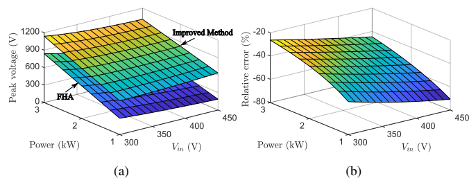
Fig. 16: LCC-S compensation. (a) Peak voltage of L_f . (b) Relative error.
