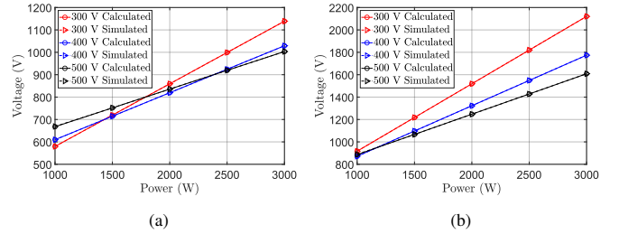
Fig. 8: LCC-S compensation, M = 105 \mu\text{H} . (a) Peak voltage of L_f . (b) Peak voltage of secondary coil.
