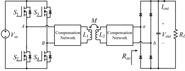
Fig. 1: Schematic of a WPT system.
