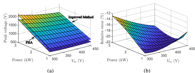
Fig. 17: LCC-S compensation. (a) Peak voltage of secondary coil. (b) Relative error.
