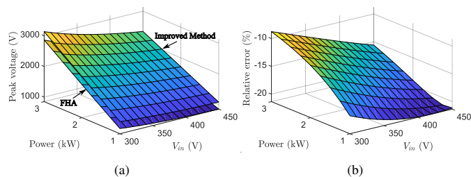
Fig. 14: S-S compensation. (a) Peak voltage of primary coil. (b) Relative error.
